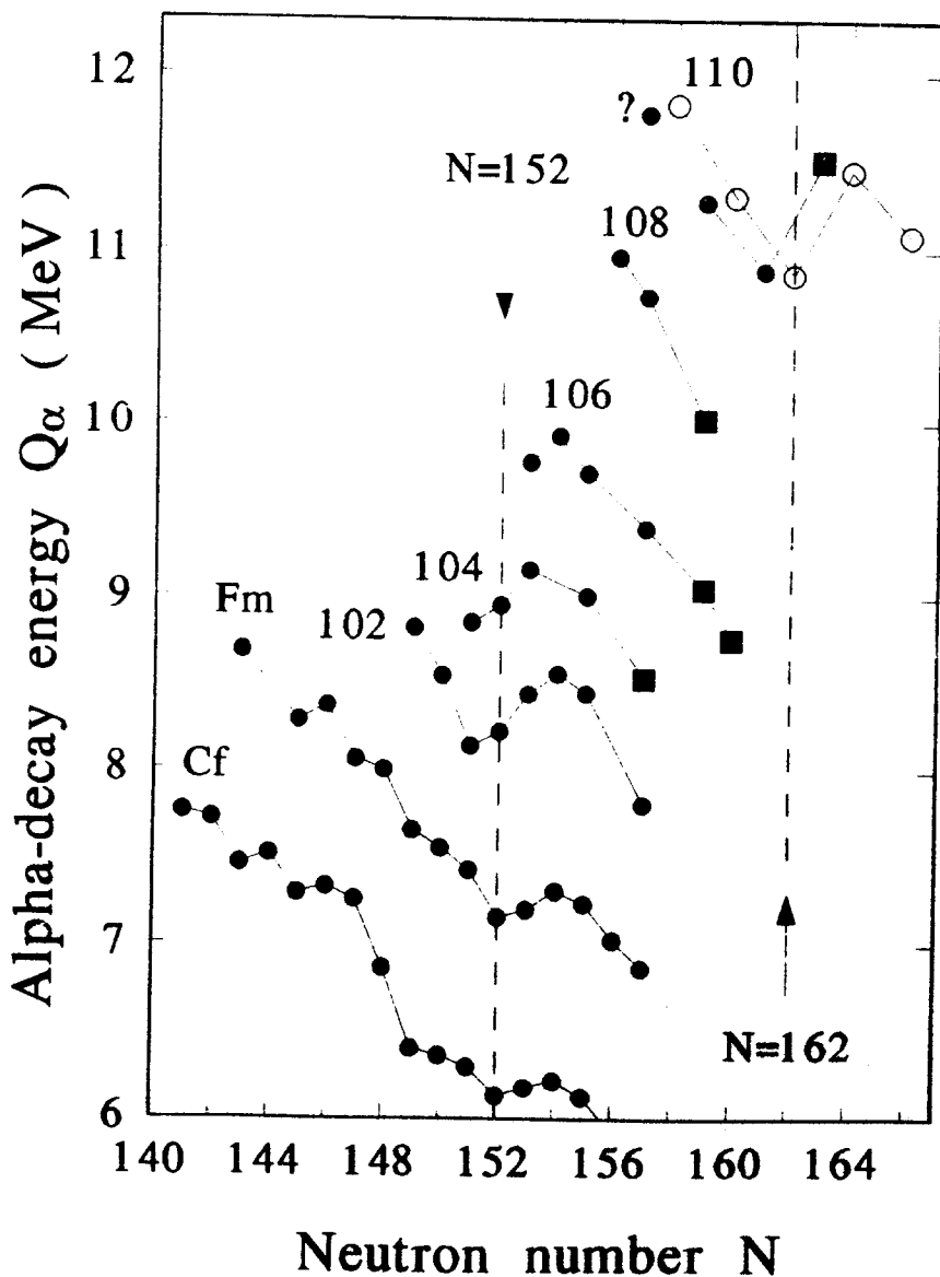
Fig.2. Alpha-decay energy Q_\alpha vs neutron number N for isotopes of even-Z elements Cf through 110 [5,6,10,11,14-17]. Squares show data from Refs. [5,6,11], as well as Q_\alpha for ^{273}110 from this work. Open circles show theoretical Q_\alpha values [4] for even-even Z=110 isotopes.
