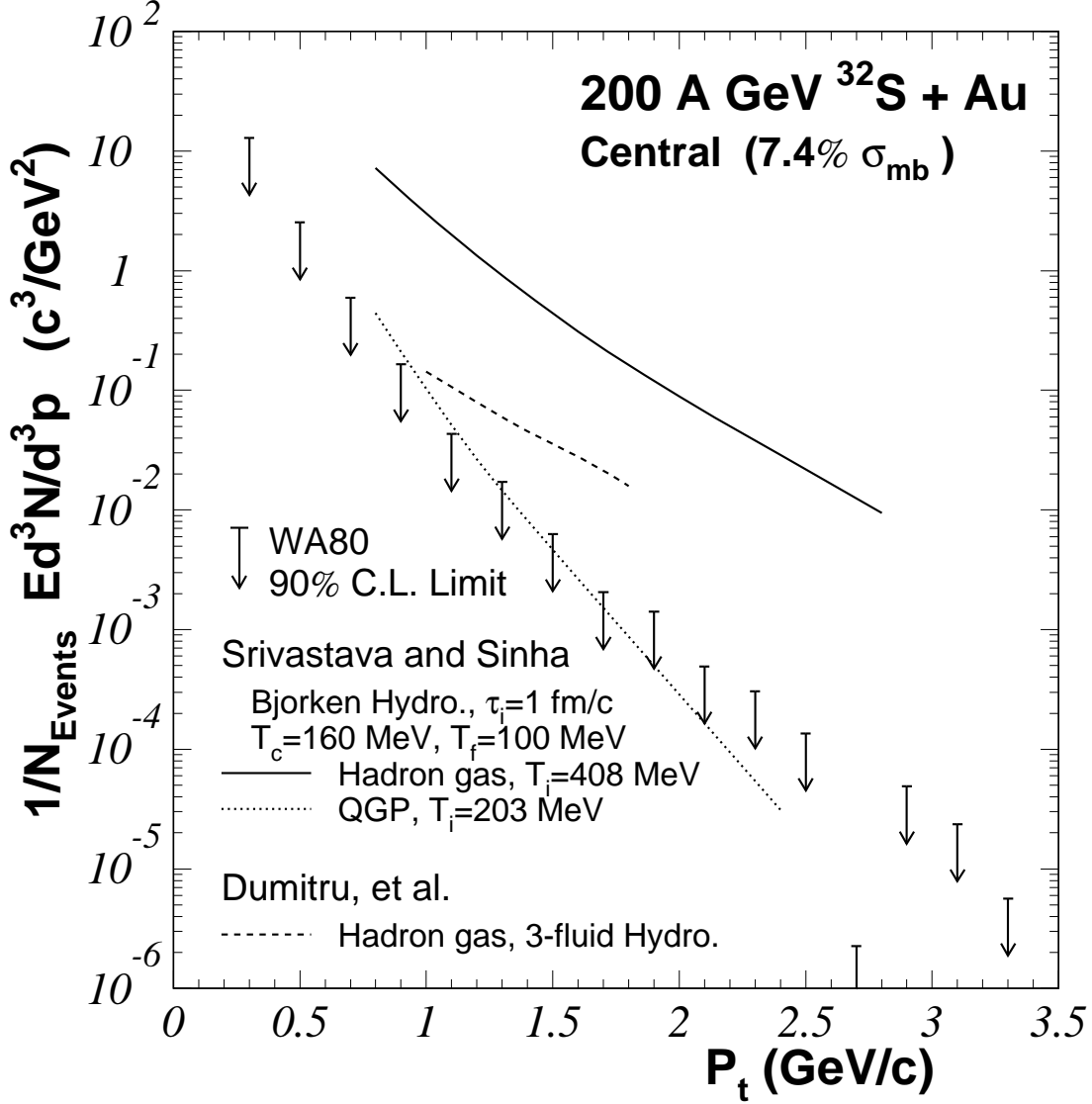
Figure 2: Upper limits at the 90% confidence level on the invariant excess photon yield per event for the 7.4% \sigma_{\text{mb}} most central collisions of 200-A GeV ^{32}\text{S} + \text{Au} . The solid curve is the calculated thermal photon production expected from a hot hadron gas taken from Ref. [5]. The dashed curve is the result of a similar hadron gas calculation taken from Ref. [7]. The dotted curve is the calculated thermal photon production expected in the case of a QGP formation also taken from Ref. [5].
