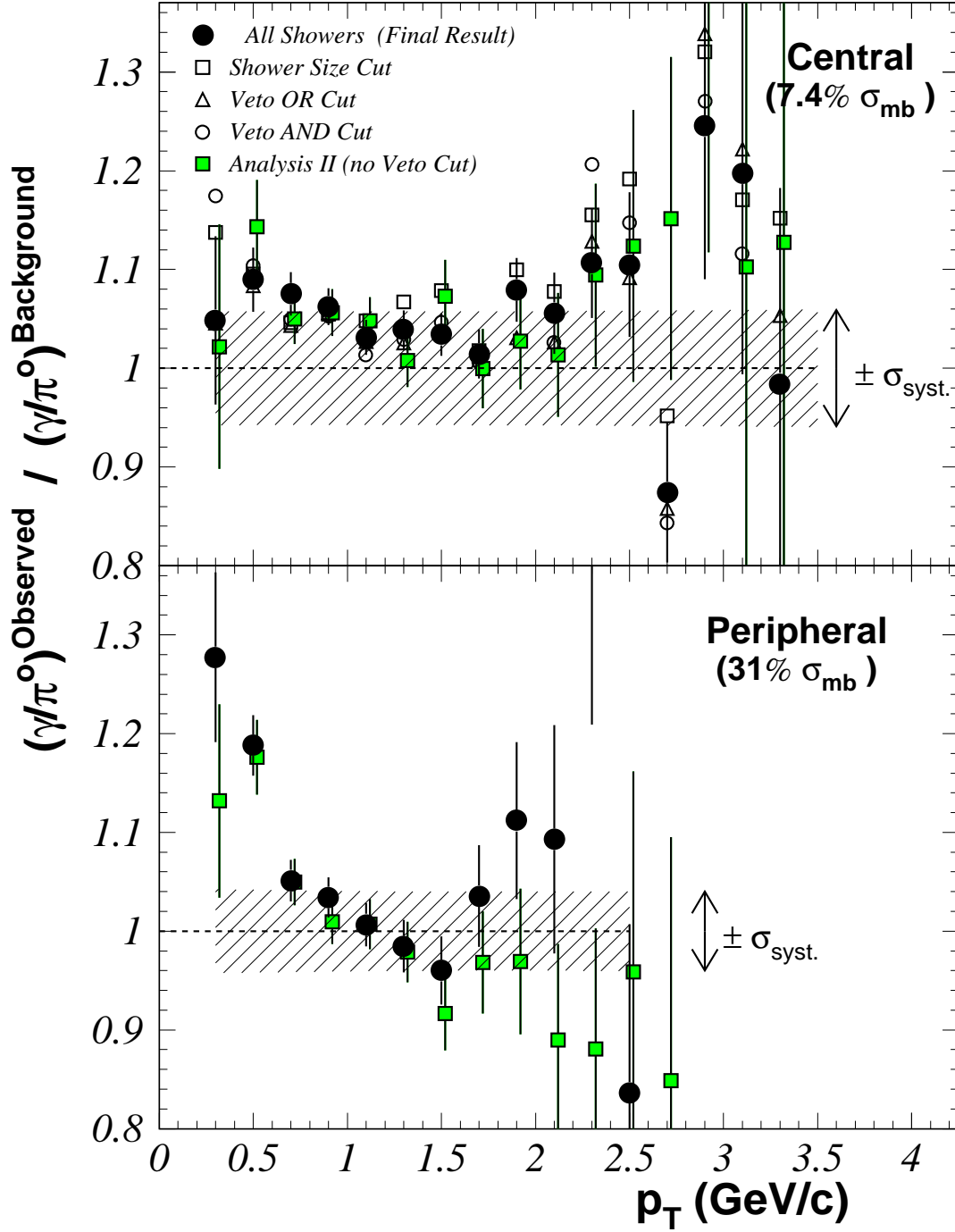
Figure 1: The ratio (\gamma/\pi^0)^{\text{obs}}/(\gamma/\pi^0)^{\text{bkgd}} as a function of transverse momentum for peripheral and central collisions of 200·A GeV ^{32}\text{S} + \text{Au} . The errors on the data points (shown for the solid points only) indicate the statistical errors only. The shaded regions indicate the total estimated p_T -dependent systematic errors which bound the region corresponding to no photon excess.
