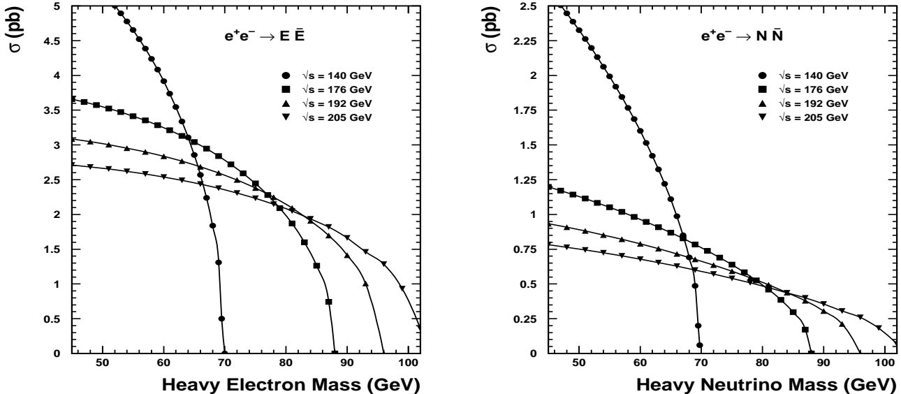
Figure 1: The total cross section (at various c.m. energies) for E^+E^- and NN\bar{} production at LEP2.
