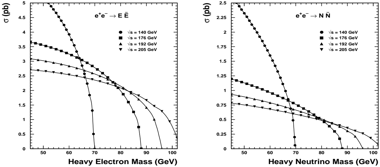
Figure 1: The total cross section (at various c.m. energies) for E^+E^- and NN̄ production at LEP2.
