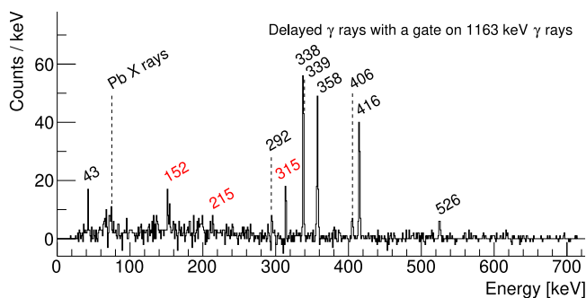
Fig. 4 | Recoil-gated background-subtracted delayed \gamma -ray energy spectrum measured at the MARA focal-plane. A gate on the 1163 keV 2_2^+ \rightarrow 0_1^+ \gamma rays has been applied. The peaks are labelled according to transition energies (new transitions in red).
