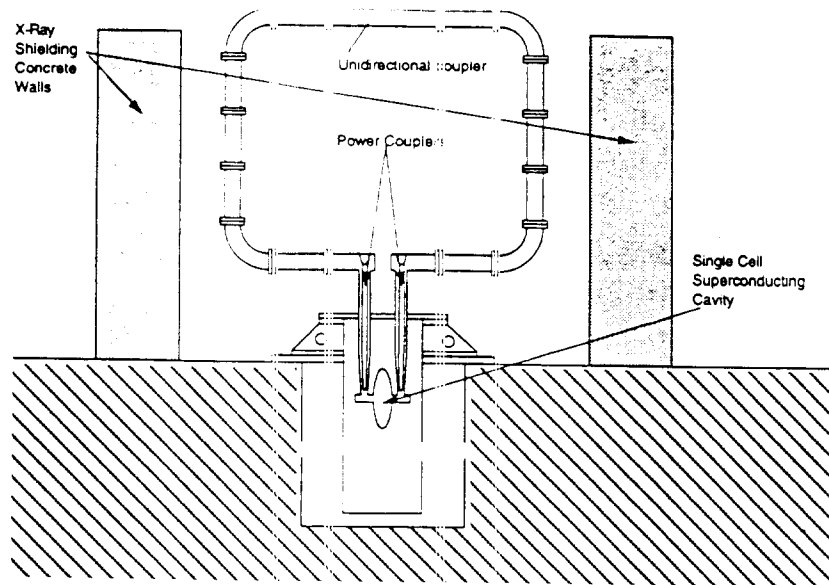
Figure 1. Resonant ring testing concept
