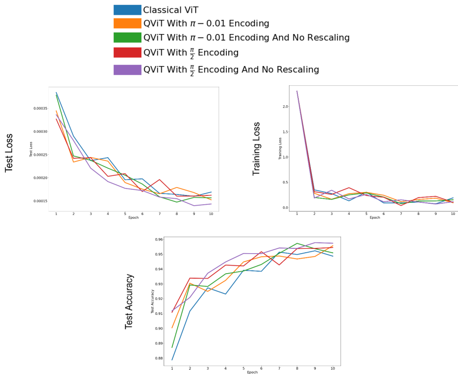
Figure 2. Plots depicting the training loss, test loss, and the test accuracy. Given the scale of the y-axis, the plots indicate that the proposed QViT is comparable in performance with the classical ViT.
