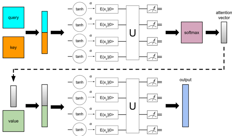
Figure 1. This figure depicts the flow of information through quantum attention, though the circuit parameters can be found in Section 3.3. The query and key matrices are flattened into vectors. The vectors are then concatenated together and are passed through a hyperbolic tangent activation function, whose outputs are then multiplied by a scalar, \alpha . The inputs enter the quantum circuit and are encoded via an encoding method, E(x_i) (where x_i is an input to the quantum circuit. Note that the illustration stops at x_4 for brevity). The above process is repeated for the value matrix whose resulting vector is concatenated with the attention vector, and the result after the imposed variational quantum circuit forms the output for Quantum Self-Attention.
