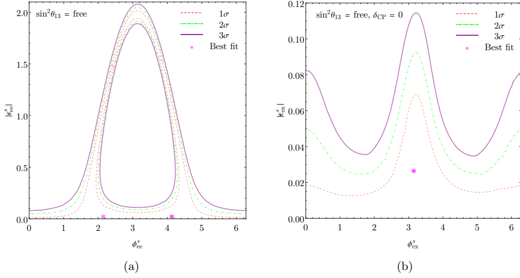
Figure 10. Allowed region in the (\phi_{e\alpha}^s, |\epsilon_{e\alpha}^s|) plane marginalizing over \sin^2 \theta_{13} for \delta_{\text{CP}} = 0 . The left panel is for \epsilon_{ee}^s , and the right for \epsilon_{ex}^s . The corresponding allowed regions for the magnitude of \epsilon_{e\mu}^s and \epsilon_{e\tau}^s are not bound. Details of the analysis can be found in section 4.2.4.
