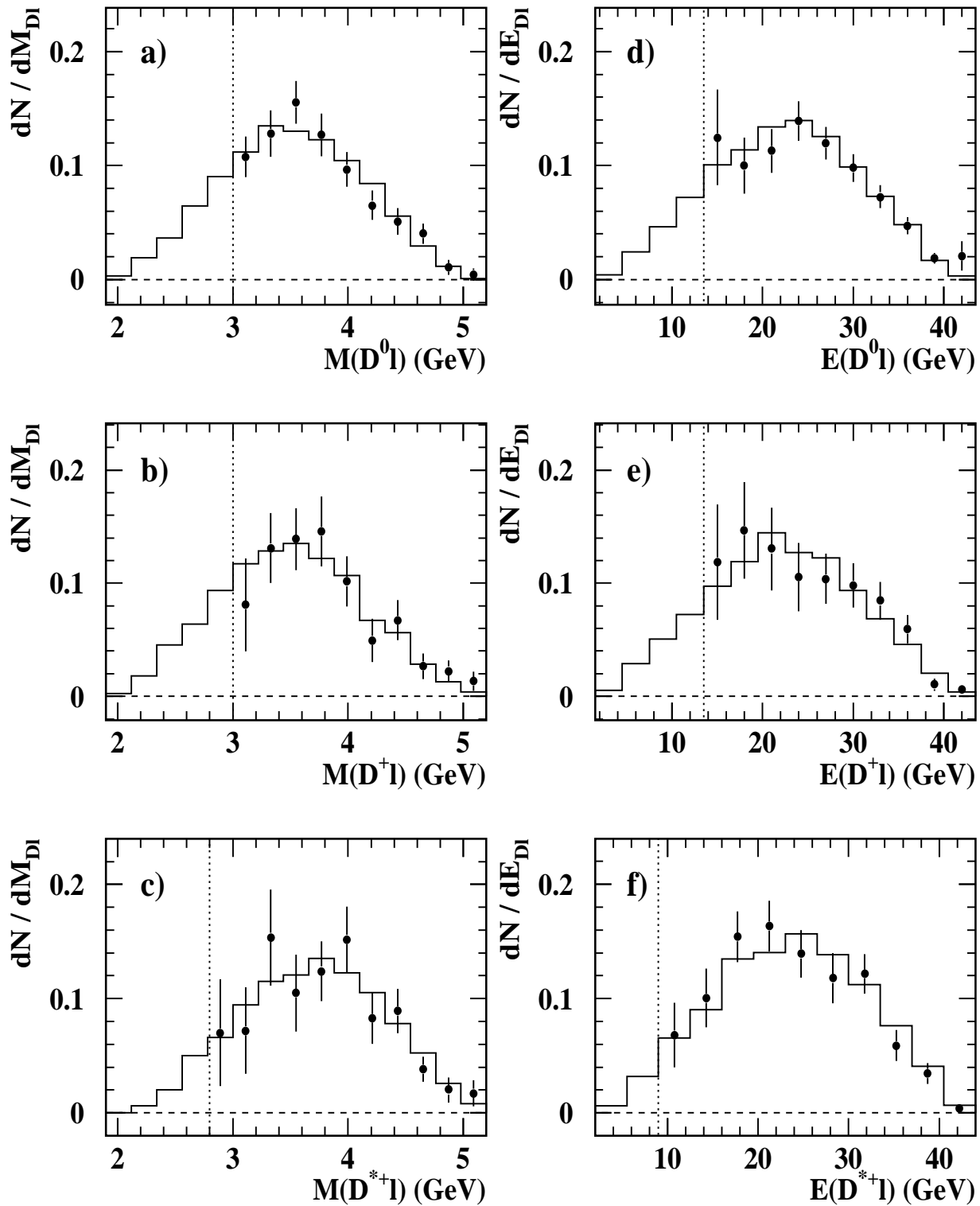
Figure 2: Monte Carlo and data comparison of M_{D\ell} for a) b \rightarrow D^0 \ell X events, b) b \rightarrow D^+ \ell X events and c) b \rightarrow D^{*+} \ell X events and E_{D\ell} for d) b \rightarrow D^0 \ell X events, e) b \rightarrow D^+ \ell X events and f) b \rightarrow D^{*+} \ell X events. The histograms are the generator level Monte Carlo distributions and the points are efficiency corrected data after background subtraction. The dotted line on each plot indicates the experimental lower limit due to the selection criteria applied. These distributions are not fitted, only normalized such that the integration over the experimental ranges are equal.
