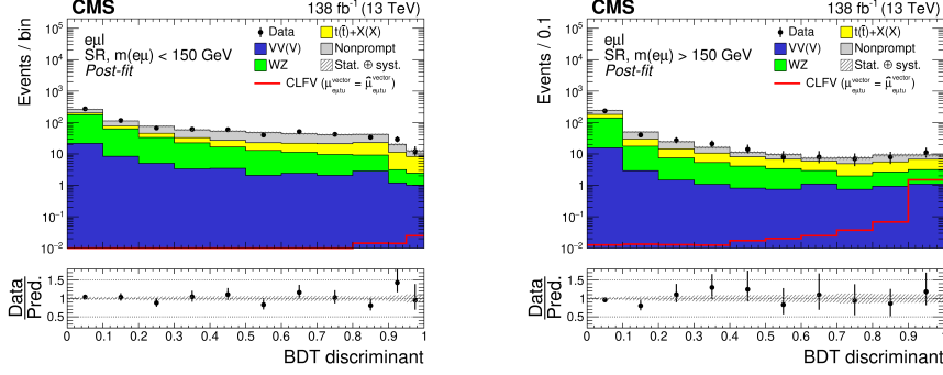
Figure 7: The BDT output and the post-fit event yields for the charged lepton flavor violation search in the low-mass (left) and high-mass (right) signal regions [4].
