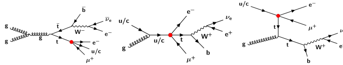
Figure 6: Feynman diagrams for the search for CLFV in the top quark sector [4].
