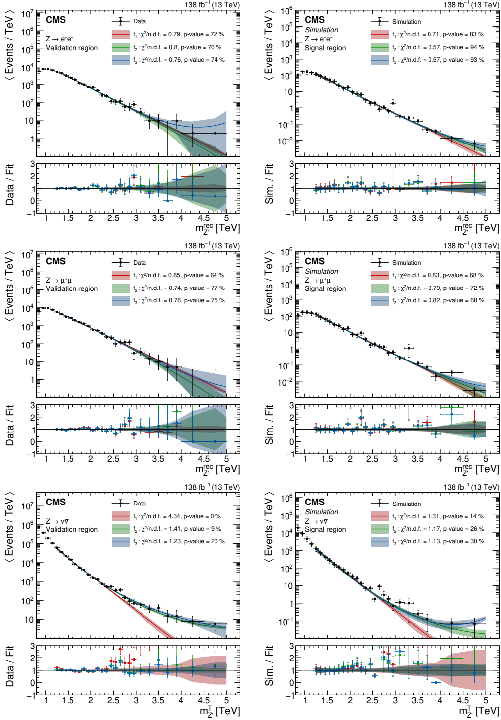
Figure 3. Fits of the background functions to the m_{Z^I} and m_{Z^T} distributions in data in the VRs (left) and simulation in the SRs (right) for the electron (upper), muon (middle), and neutrino (lower) channels. The number of events in each bin is divided by the bin width. In the panels below the distributions, the ratios of data to the background functions are displayed. The ratios to the functions f_1 , f_2 , and f_3 , are shown by red, green, and blue points, respectively. The shaded colored areas represent the statistical uncertainty from the fit. The \chi^2 values per number of degrees of freedom ( \chi^2/n.d.f. ) and the corresponding p -values are provided for each fit.
