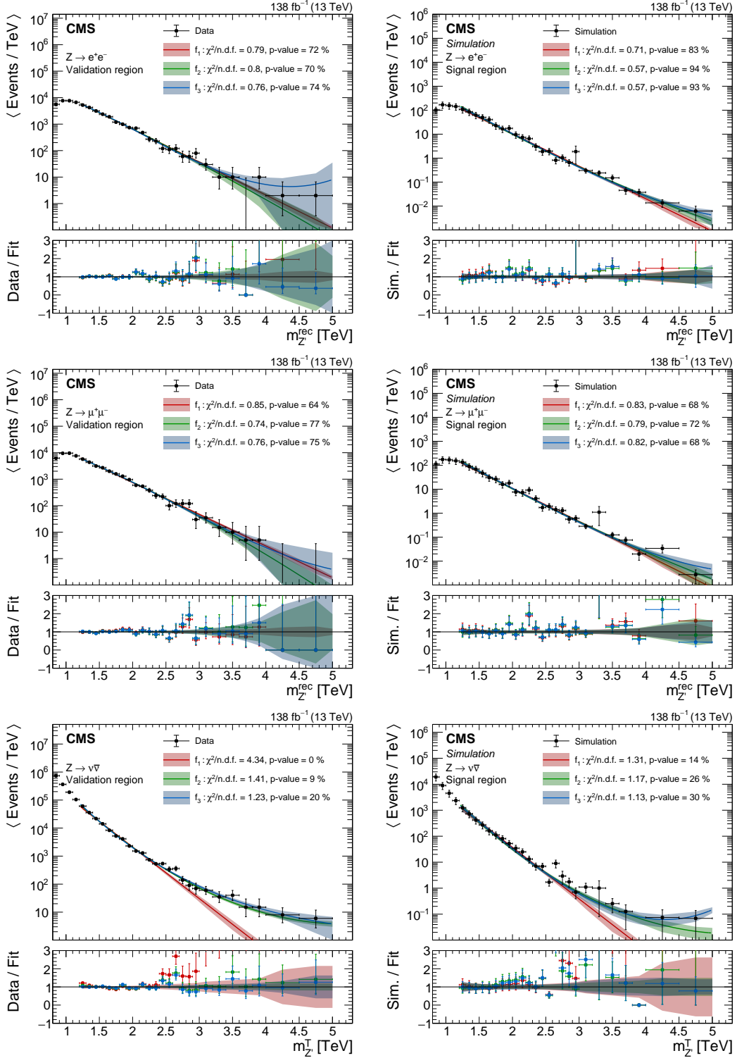
Figure 3: Fits of the background functions to the m_{Z'} and m_{Z'I}^T distributions in data in the VRs (left) and simulation in the SRs (right) for the electron (upper), muon (middle), and neutrino (lower) channels. The number of events in each bin is divided by the bin width. In the panels below the distributions, the ratios of data to the background functions are displayed. The ratios to the functions f_1 , f_2 , and f_3 , are shown by red, green, and blue points, respectively. The shaded colored areas represent the statistical uncertainty from the fit. The \chi^2 values per number of degrees of freedom ( \chi^2/n.d.f. ) and the corresponding p -values are provided for each fit.
