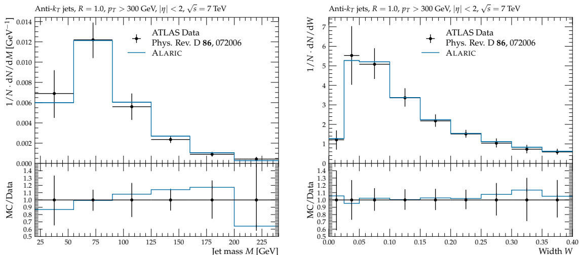
Figure 6. Jet mass and jet width measured by the ATLAS collaboration [132] at \sqrt{s} = 7 TeV, compared to predictions from ALARIC using the setup of [130].
