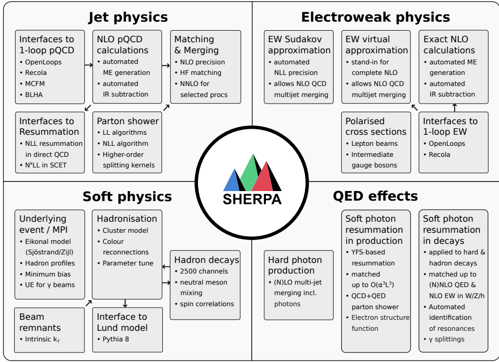
Figure 2. Schematic overview of the physics effects simulated by SHERPA, as well as major characteristics of their implementation in the event generator.
