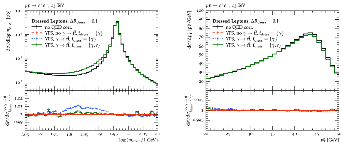
Figure 9. The dressed dilepton invariant mass m_{e^+e^-} (left) and electron transverse momentum p_T^e (right) in Drell-Yan production as described at leading order (black), by the YFS soft-photon resummation at YFS+NLO QED+NLO EW accuracy without photon-splitting corrections (red) or additionally resolving the photons further into pairs of charged particles (blue and green), including mitigating effects of adequately improved dressing strategies. For details see [218].
