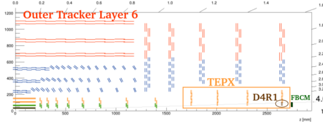
Figure 3: Location of four Phase-2 luminosity subsystems on tracker layout
