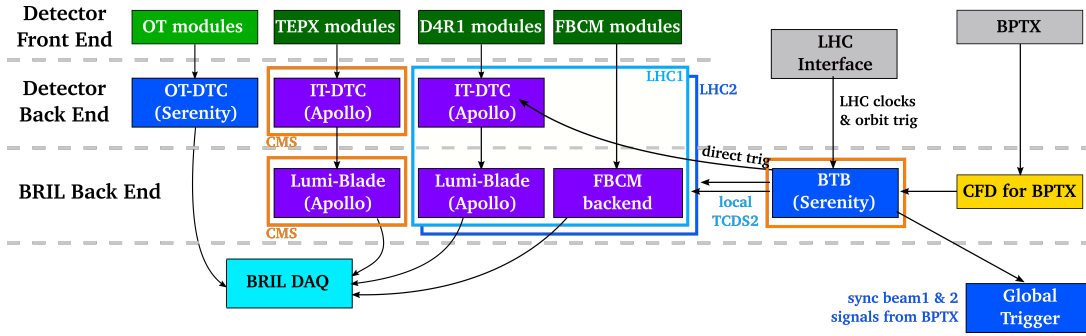
Figure 2: Simplified Schematic of the BRIL Trigger Board in relation to other BRIL and CMS subsystems
