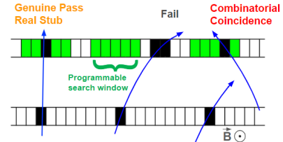
Figure 4: Representation of stub counting in OT6
