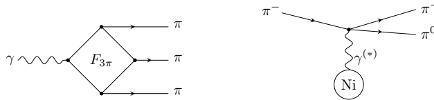
Fig. 1. – On the left: tree-level diagram of the anomalous coupling of one photon to three pions. The coupling strength is described by the chiral anomaly constant F_{3\pi} . On the right: Primakoff reaction, in which an ultra-relativistic beam pion scatters in the Coulomb field of a nucleus giving rise to the photon, three pion vertex.
