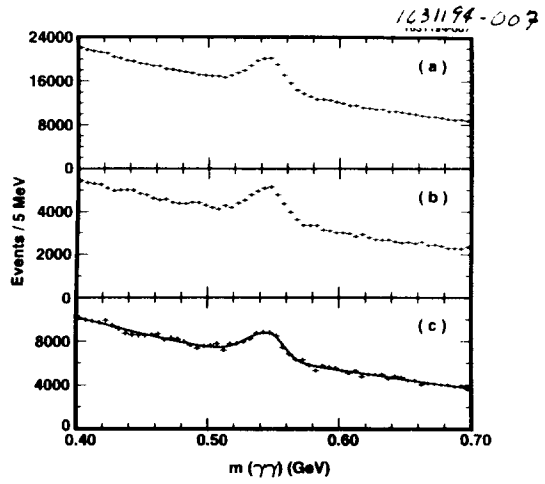
FIG. 3. The \gamma\gamma mass spectra for (a) T(4S) data, (b) continuum data, and (c) scaled continuum subtracted. The \eta momentum interval is 0.8 to 2.0 GeV/c.
