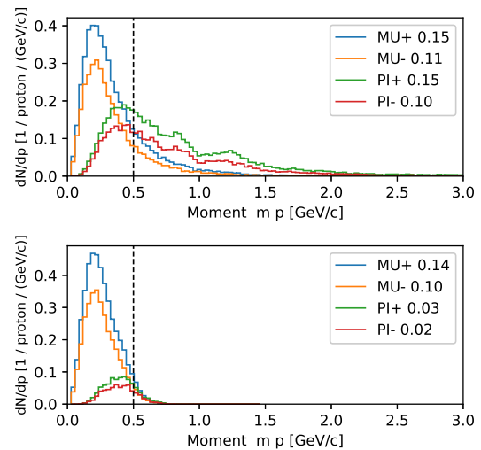
Figure 2: Momentum distribution of pions and muons entering (top) and leaving (bottom) the chicane. The chicane suppresses the higher-momentum component above \sim 0.5 GeV/c (dashed line). The numbers in the legend correspond to the pion/muon yield per primary proton.
