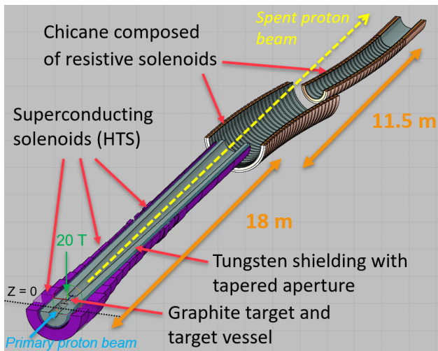
Figure 1: FLUKA model for radiation studies.
