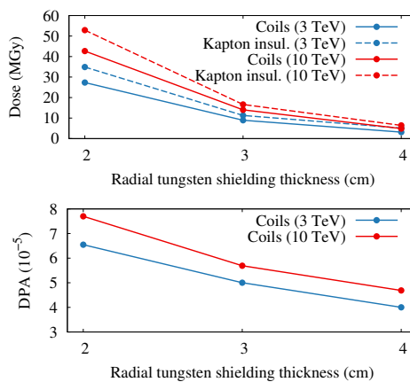
Figure 5: Maximum dose in the cold bore insulation and in the coils (top), and maximum Displacement Per Atom (DPA) in the coils (bottom). The figures assume 5 years of operation with about 140 days of running time per year.
