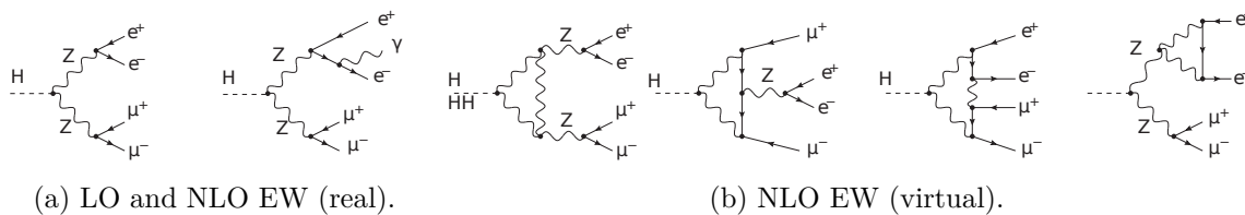
Figure 3. Sample diagrams contributing to the Higgs-boson decay into four charged leptons. A tree-level diagram is shown (a, left), along with a real-radiation (a, right) and one-loop diagrams (b).
