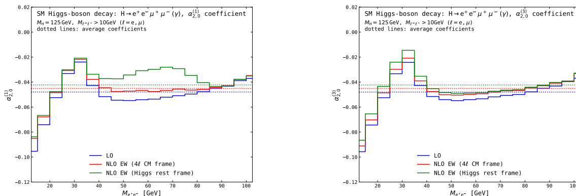
Figure 4. Dependence of the polar coefficients \alpha_{2,0}^{(1)} (left plot, associated to Z^{(*)} \rightarrow e^+e^- ) and \alpha_{2,0}^{(3)} (right plot, associated to Z^{(*)} \rightarrow \mu^+\mu^- ) on the off-shell-ness of the e^+e^- pair ( M_{e^+e^-} ), in the Higgs-boson decay into four charged leptons (see eq. (3.5)) at LO and NLO EW accuracy. In the case of NLO EW results, two different choices are made for the reference frame where polarisations of intermediate Z^{(*)} bosons are defined: the four-lepton CM frame (red) and the Higgs-boson rest frame (green). Dashed lines are reference values obtained integrating over M_{e^+e^-} .
