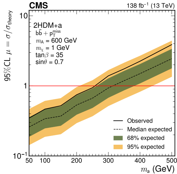
Figure 7: The 95% CL upper limit on the signal strength modifier of DM produced in association with a pair of bottom quarks for m_A = 600 GeV, \sin\theta = 0.7 , m_\chi = 1 GeV, and \tan\beta = 35 , for the combination of SR1 and SR2. The green and yellow bands show the \pm 1 and \pm 2 standard deviations from expected limits. The mass points below the red line are excluded.
