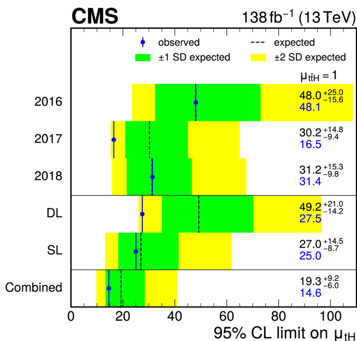
Figure 13. Observed (solid vertical line) and expected (dashed vertical line) upper 95% CL limit on the tH signal strength modifier \mu_{tH} for different channels and years, where the uncertainties are uncorrelated between the channels and years, and in their combination. The green (yellow) areas indicate the one (two) standard deviation confidence intervals on the expected limit.
