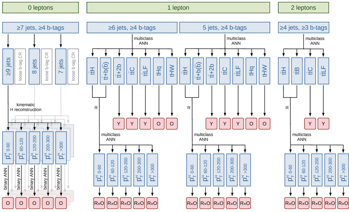
Legend: ■ Distribution in template fit, event yield (Y), ANN output (O), likelihood ratio of ANN outputs (R), product of likelihood ratio of ANN outputs and STXS ANN output (R x O)
