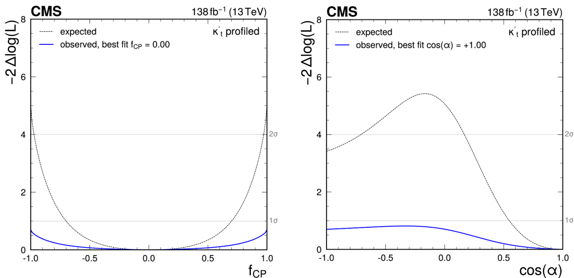
Figure 17. Observed (solid blue line) and expected (dotted black line) likelihood ratio test statistic as a function of f_{CP} (left) and \cos \alpha (right), where \kappa_V is 1 and \kappa'_t = \sqrt{\tilde{\kappa}_t^2 + \kappa_t^2} , the overall modifier of the top-Higgs coupling strength, is profiled.
