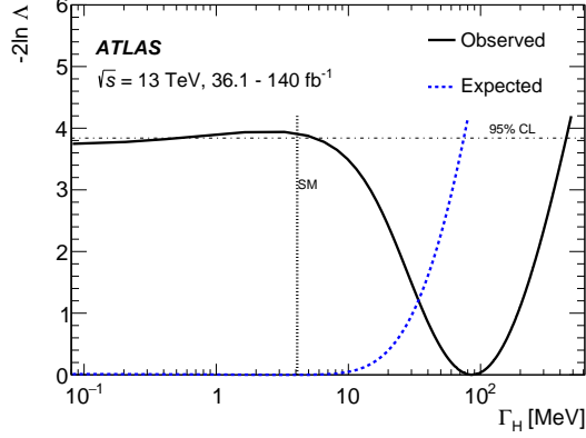
Figure 2: The observed (expected) profile likelihood ratio, -2 \ln \Lambda , as a function of \Gamma_H is shown as a solid (dashed) line. The Higgs-top Yukawa coupling strength \kappa_t and other Higgs boson coupling strength parameters as described in Section 3 are profiled. The 95% confidence interval is indicated by the intersections of the horizontal line with the -2 \ln \Lambda curves. The vertical line indicates the SM prediction.
