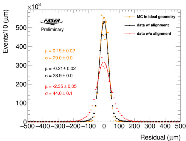
Fig. 11. Distribution of residuals from the tracks reconstructed from MC simulation in ideal geometry (orange), from data in original geometry (red), and data in aligned geometry (black) with an integrated luminosity of 596 pb -1 .
