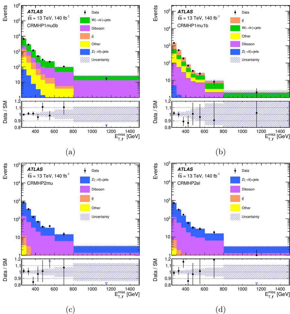
Figure 2. Distribution of E_{T,\ell}^{\text{miss}} after the background-only fit, in the control regions: (a) CRMHP1mu0b, (b) CRMHP1mu1b, (c) CRMHP2mu, and (d) CRMHP2e1. The total uncertainty in the background is shown as a shaded band and the error bars on the data points represent the statistical uncertainty. Small background contributions such as ttV , Vh , single-top and triboson processes are grouped into one category and shown as “Other”. The last bin contains the overflow.
