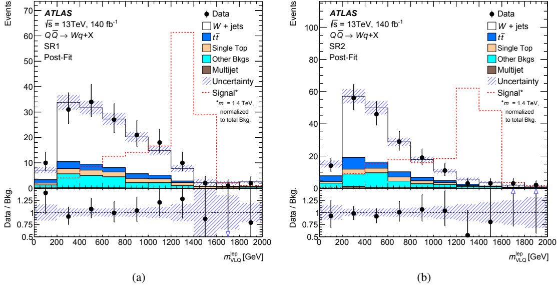
Figure 4: Distribution for the reconstructed mass of the leptonically decaying VLQ, m_{VLQ}^{lep} , in (a) SR1 and (b) SR2 after the fit using the background-only hypothesis. For comparison, the shape of the VLQ signal distribution is overlaid for \mathcal{B}(Q \rightarrow Wq) = 1 with m_{VLQ} = 1400 GeV and normalized to the total background. The uncertainty bands include all systematic uncertainties described in Section 7. An arrow in the bottom panel indicates that the given data point falls outside the range of the plot.
