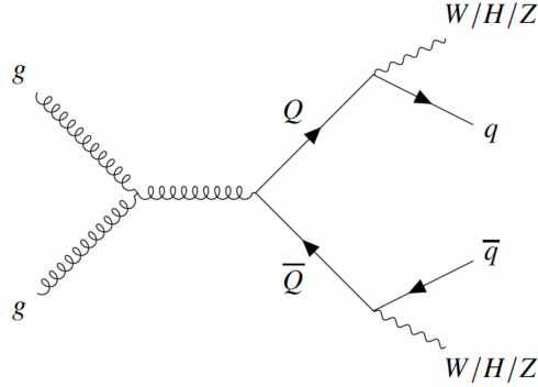
Figure 1: Illustrative Feynman diagram of pair production of the vectorlike quarks. Each vectorlike quark decays into a light quark and either a W boson, a Z boson, or a Higgs boson.
