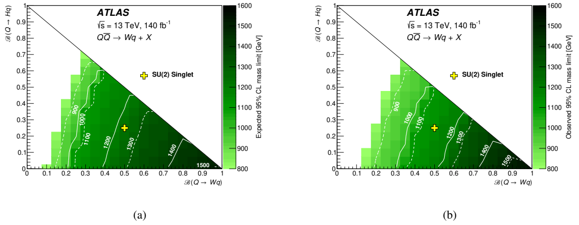
Figure 6: (a) Expected and (b) observed lower limit on the VLQ mass for various branching ratio ( \mathcal{B} ) configurations at 95% CL. The x -axis shows the branching ratio for decay to a W boson, while the y -axis shows the branching ratio for decay to a Higgs boson. The branching ratio to a Z boson is determined by the requirement that \mathcal{B}(Q \rightarrow Zq) = 1 - \mathcal{B}(Q \rightarrow Wq) - \mathcal{B}(Q \rightarrow Hq) . The white region above the solid black line is excluded due to the sum of the individual branching ratios being greater than one. In the white region below this line the lower limit on the VLQ mass is below 800 GeV. The yellow marker indicates the branching ratios for the SU(2) singlet scenario.
