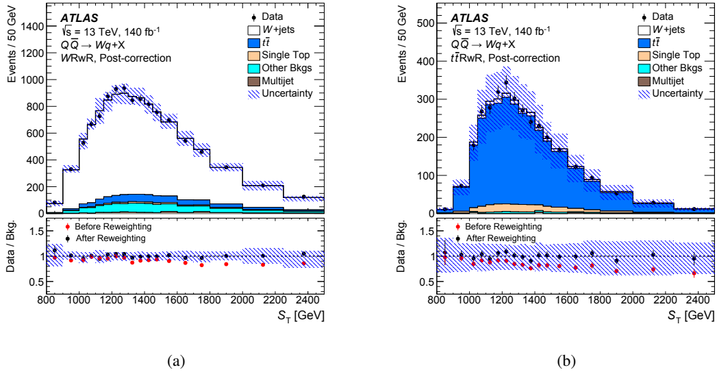
Figure 2: Reconstructed S_T distribution in the (a) WRwR and (b) t\bar{t} RwR after applying the reweighting corrections. The uncertainty band includes all systematic uncertainties, as described in detail in Section 7. The lower panel shows the ratio of data to the SM prediction before (red points) and after (black points) applying the reweighting corrections.
