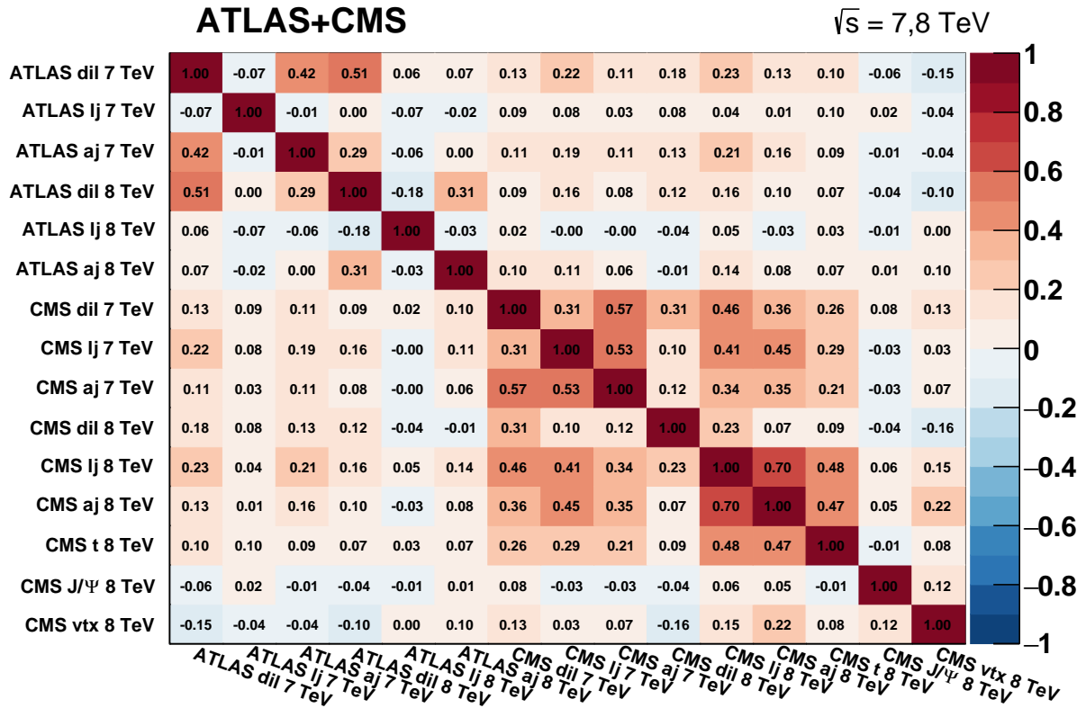
Figure A.2: Correlation matrix for the ATLAS and CMS 7 and 8 TeV m_t measurements in the dilepton (‘‘dil’’), lepton+jets (‘‘lj’’), and all-jets (‘‘aj’’) channels, and for the CMS 8 TeV m_t measurements in the single top (‘‘t’’), secondary vertex (‘‘vtx’’), and J/\psi analysis (‘‘ J/\psi ’’).
