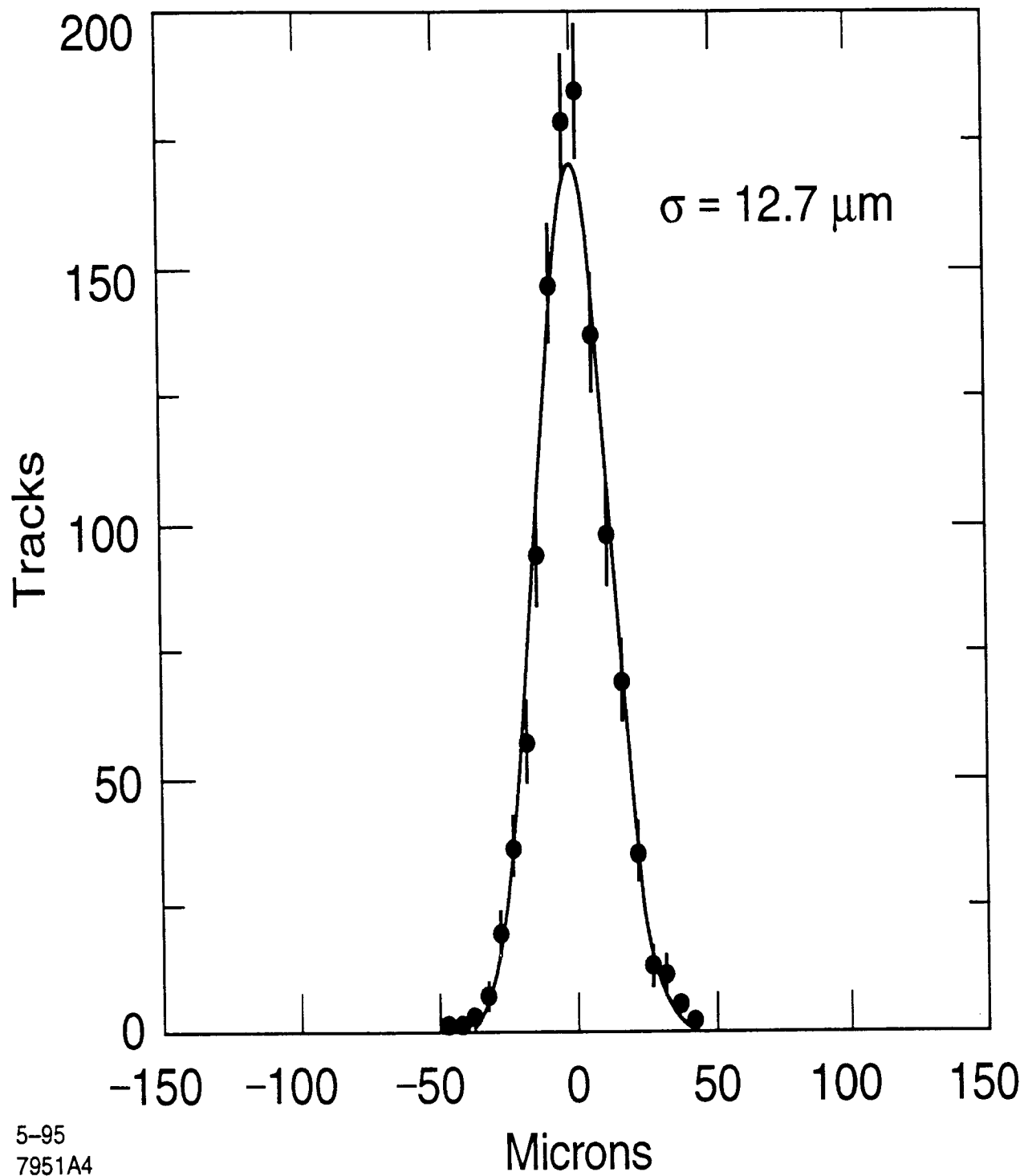
Figure 4: Distribution of track impact parameters in \mu^+\mu^- events with respect to the \langle IP \rangle determined from hadronic events.
