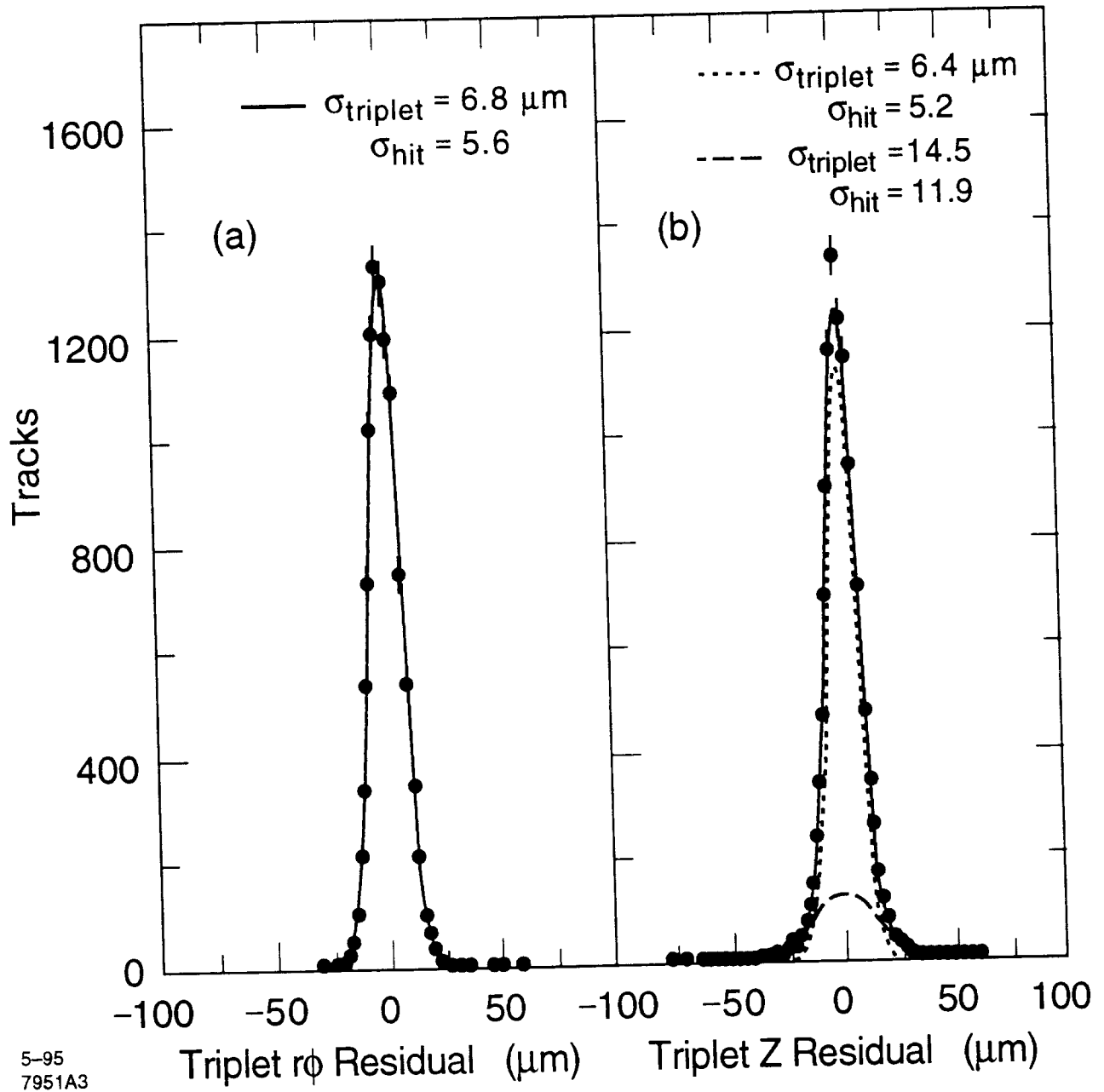
Figure 3: Plot of the residual of the middle hit in a triplet of VXD hits from the same track on three separate layers relative to track which is forced to go through the first and last hit of the triplet. All tracks with momentum greater than 1 GeV/c for all \cos\theta in hadronic Z^0 events are used. The single hit resolution ( \sigma_{\text{hit}} ) is obtained from the triplet miss distance by dividing by 1.22 to account for broadening due to the finite resolution of the other two hits at an average lever arm ratio.
