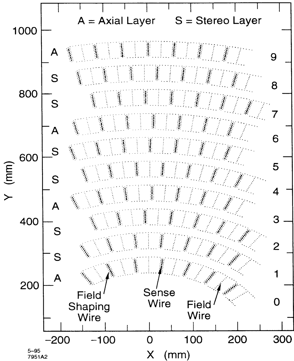
Figure 2: xy cross-section of a portion of the CDC endplate showing the relative location of sense and field wires.
