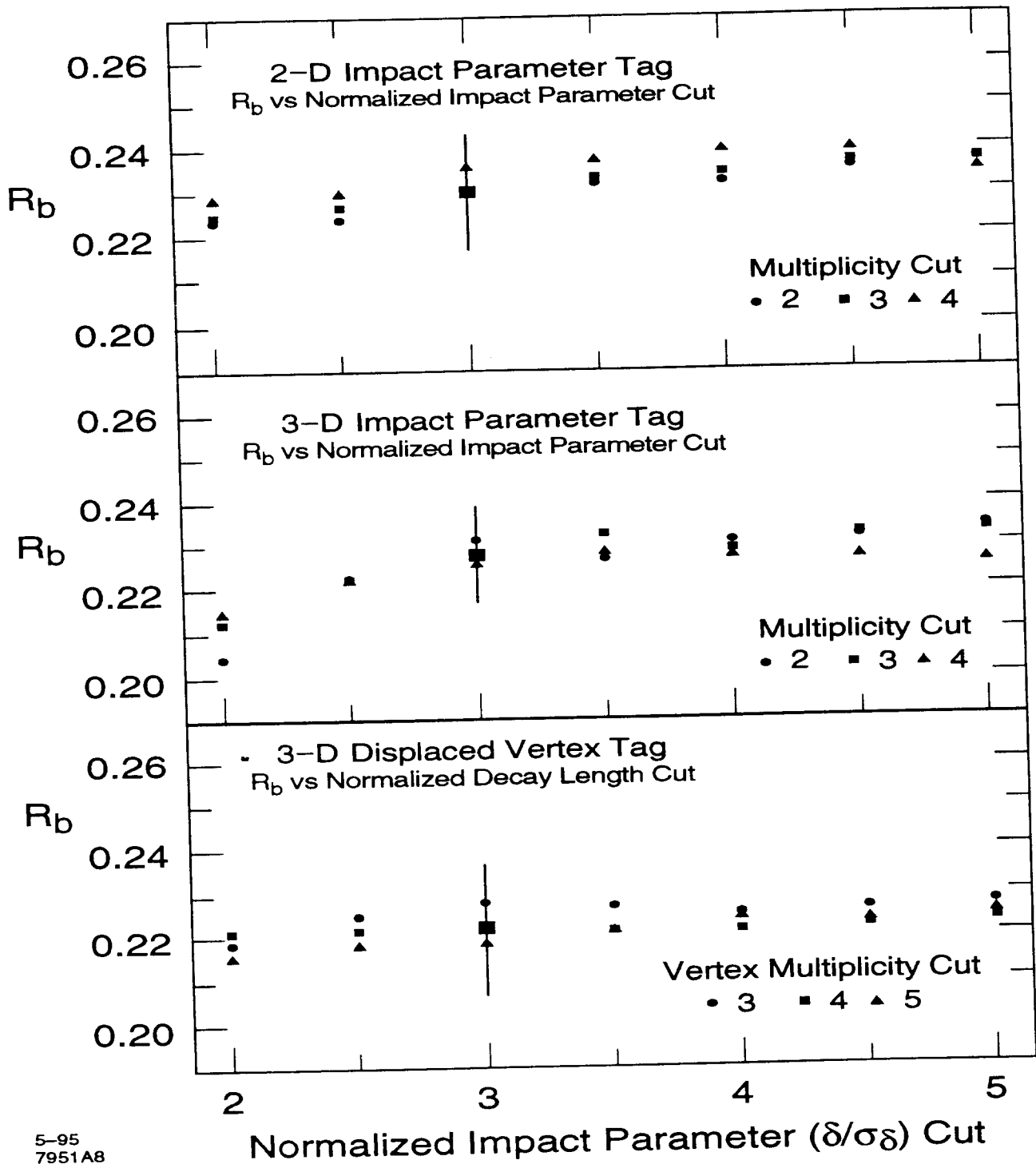
Figure 8: R_b versus tagging cuts in the 2-D and 3-D Impact Tag and the 3-D Displaced Vertex Tag. The result at nominal cuts for each method is shown as large square together with the estimated total error bar at the nominal cuts.
