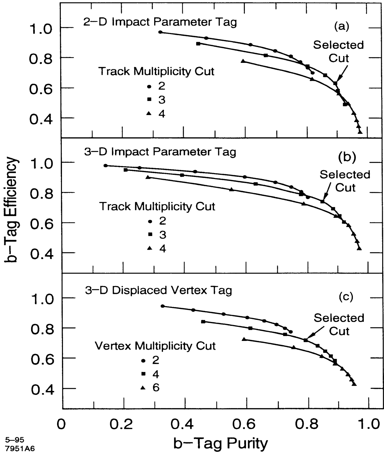
Figure 6: b\bar{b} event tagging efficiencies versus purities for each b\bar{b} event tagging method with different multiplicity and significance cuts, derived from the Monte Carlo. Each curve represents the estimated efficiencies and purities as the significance cut is varied from 1.5 to 5.0, in steps of 0.5, while the multiplicity cut is fixed.
