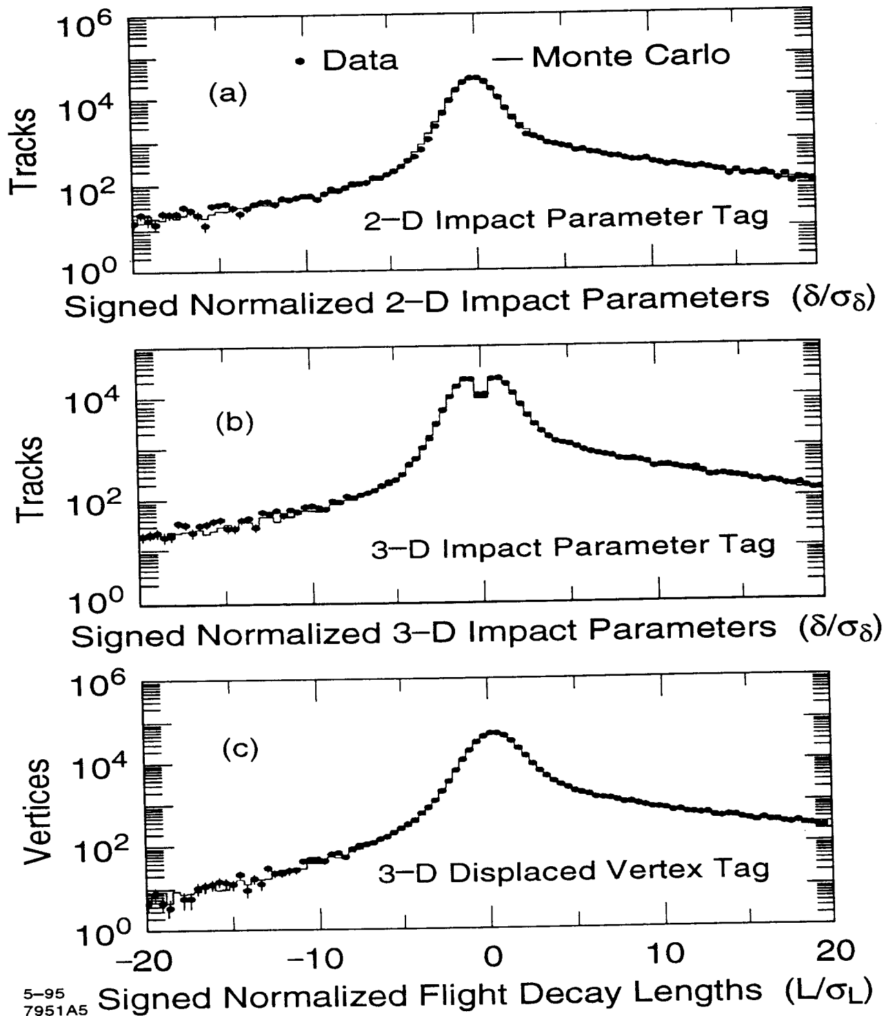
Figure 5: Data and Monte Carlo Signed Normalized 2-D and 3-D Impact Distributions, and Signed Normalized Flight Decay Length Distributions without tracking resolution corrections for the MC.
