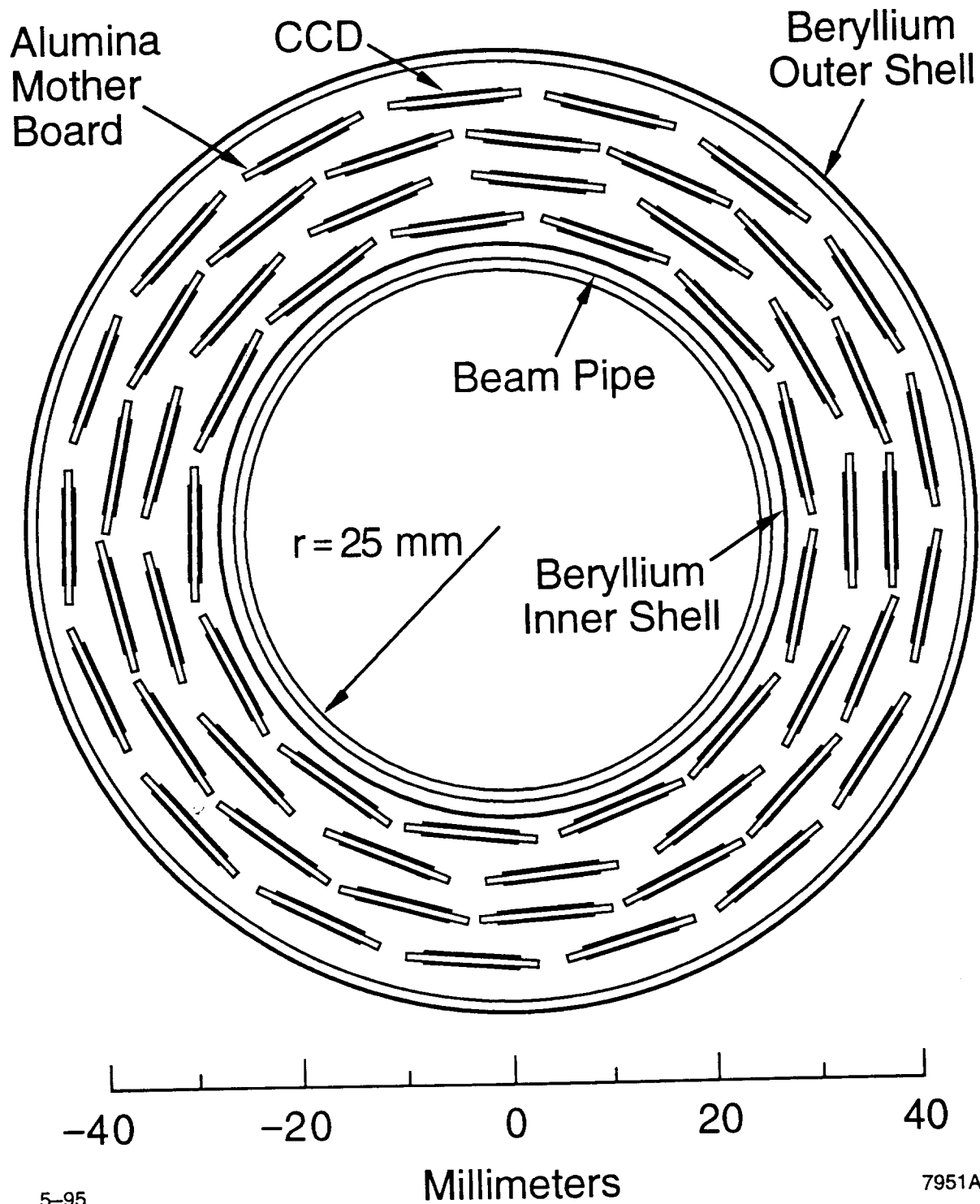
Figure 1: xy cross-section of the VXD geometry. There are 60 ladders with 4 CCDs on the top face and 4 CCDs on the bottom face of each ladder.
