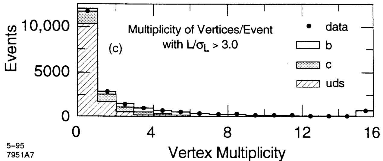
Figure 7: Data and Monte Carlo event counts vs. number of significant tracks and vertices in the events. The Monte Carlo total event count has been normalized to data.
