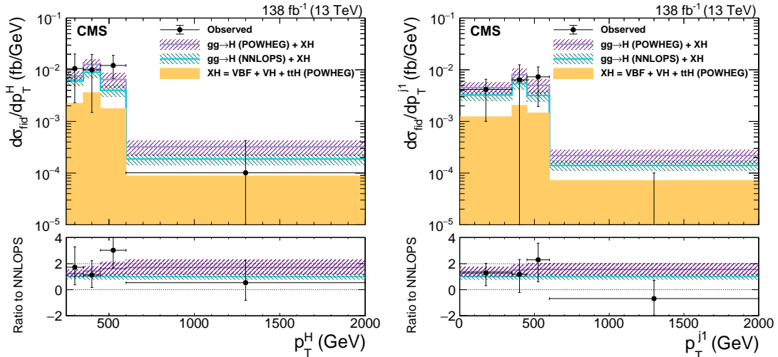
Figure 3: Observed and expected differential fiducial cross sections in bins of p_T^H (left) and p_T^j (right). The last bins include the overflow. The uncertainty bands in the theoretical predictions include uncertainties from the following sources: PDF, renormalization and factorization scales, underlying event and parton showering, and the branching fraction \mathcal{B}(H \rightarrow \tau\tau) .
