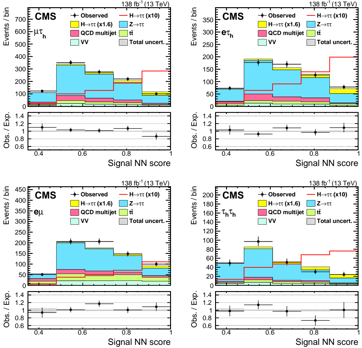
Figure 2: Observed and expected NN distributions in the signal-enriched region, after combining all four p_T^H bins, in the \mu\tau_h (upper left), e\tau_h (upper right), e\mu (lower left), and \tau_h\tau_h (lower right) channels. The signal and background distributions are the result of a simultaneous binned maximum likelihood fit to all three output NN distributions, including all individual p_T bins and data-taking years. The bottom panel shows the ratio of the number of events observed in data to that of the expected background.
