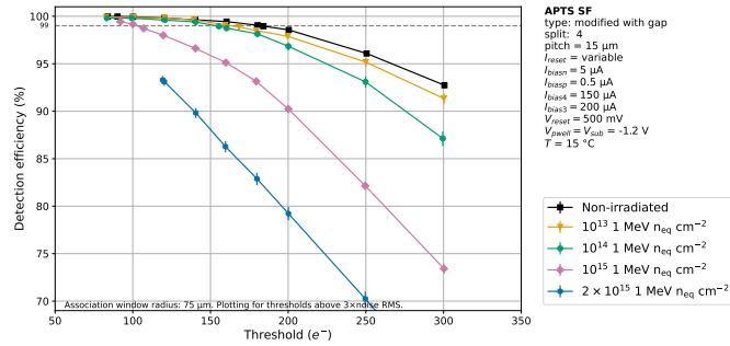
Figure B.31: Efficiency comparison between different NIEL irradiation levels as a function of the applied seed threshold. Chiller temperature was 15 \text{ }^\circ\text{C} . APTS with 15 \text{ }\mu\text{m} pitch, modified with gap, split 4, reference variant, V_{\text{sub}} = -1.2 \text{ V} .
