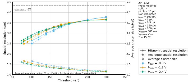
Figure B.39: Resolution comparison between different reverse substrate voltages as a function of the applied seed threshold. APTS with 15 µm pitch, modified, split 4, reference variant.
