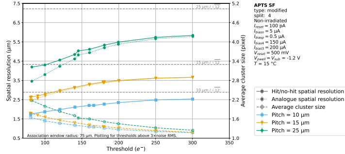
Figure B.42: Resolution comparison between different pitches as a function of the applied seed threshold. APTS with modified, split 4, reference variant, V_{\text{sub}} = -1.2 \text{ V} .
