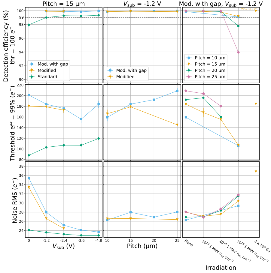
Figure 14: Comparison of the main characteristics extracted from the efficiency plots versus threshold. APTS with split 4, reference variant.
