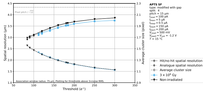
Figure B.46: Resolution comparison with TID irradiated APTS as a function of the applied seed threshold. Chiller temperature was 15 °C. APTS with 15 \mu\text{m} pitch, modified with gap, split 4, reference variant, V_{\text{sub}} = -1.2 \text{ V} .
