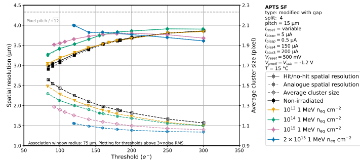
Figure B.43: Resolution comparison between different NIEL irradiation levels as a function of the applied seed threshold. Chiller temperature was 15 \text{ }^\circ\text{C} . APTS with 15 \mu\text{m} pitch, modified with gap, split 4, reference variant, V_{\text{sub}} = -1.2 \text{ V} .
