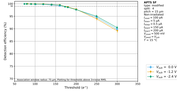
Figure B.27: Efficiency comparison between different reverse substrate voltages as a function of the applied seed threshold. APTS with 15 \mu\text{m} pitch, modified, split 4, reference variant.
