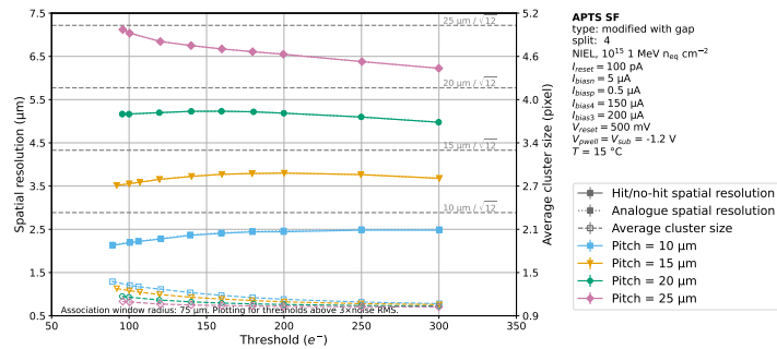
Figure B.47: Resolution comparison between different pitches as a function of the applied seed threshold for a NIEL irradiation level of 10^{15} 1 MeV n_{\text{eq}} \text{ cm}^{-2} . Chiller temperature was 15 °C. APTS with modified with gap, split 4, reference variant, V_{\text{sub}} = -1.2 \text{ V} .
