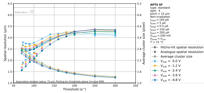
Figure B.40: Resolution comparison between different reverse substrate voltages as a function of the applied seed threshold. APTS with 15 µm pitch, standard, split 4, reference variant.
