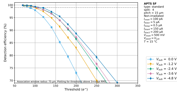
Figure B.28: Efficiency comparison between different reverse substrate voltages as a function of the applied seed threshold. APTS with 15 \mu\text{m} pitch, standard, split 4, reference variant.
