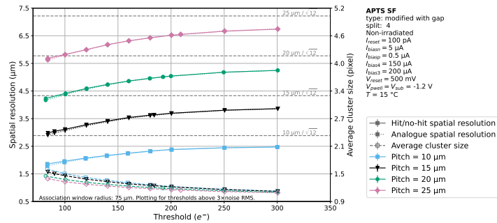
Figure B.41: Resolution comparison between different pitches as a function of the applied seed threshold. APTS with modified with gap, split 4, reference variant, V sub = -1.2 V.
