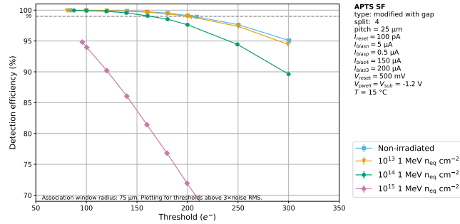
Figure B.33: Efficiency comparison between different NIEL irradiation levels as a function of the applied seed threshold. Chiller temperature was 15 °C. APTS with 25 μm pitch, modified with gap, split 4, reference variant, V_{sub} = -1.2 \text{ V} .
