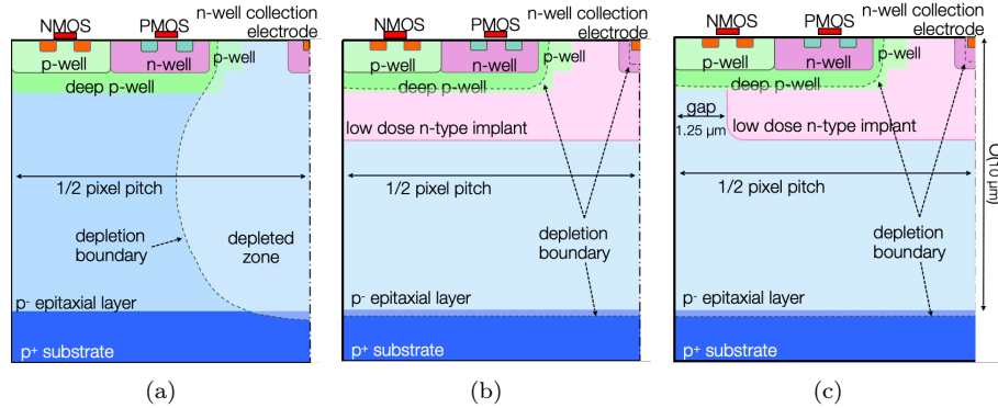
Figure 2: Cross-sections of three different pixel designs implemented: (a) standard: no additional low-dose implant, (b) modified: with deep blanket low dose n-type implant, and (c) modified with gap: with a gap in the deep low dose n-type implant at the pixel borders.
