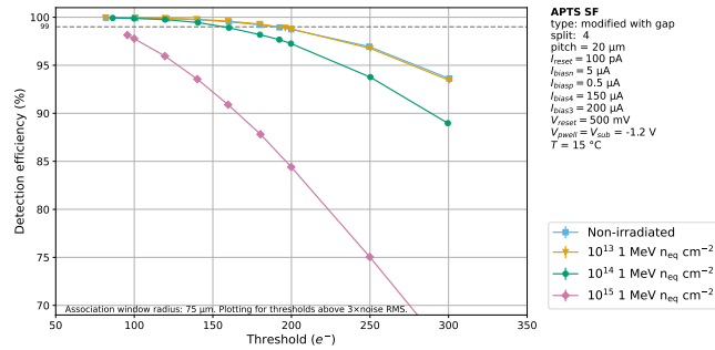
Figure B.32: Efficiency comparison between different NIEL irradiation levels as a function of the applied seed threshold. Chiller temperature was 15 \text{ }^\circ\text{C} . APTS with 20 \text{ }\mu\text{m} pitch, modified with gap, split 4, reference variant, V_{\text{sub}} = -1.2 \text{ V} .
