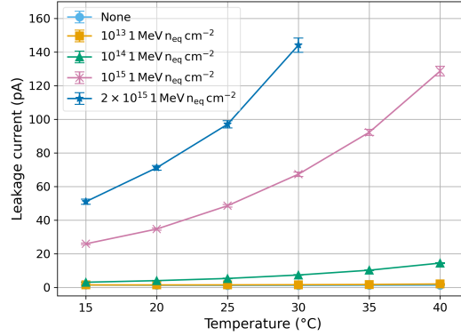
Figure 7: Leakage current versus temperature for different irradiation levels at a reverse substrate bias of 1.2 V. APTS with 15 \mu\text{m} pitch, modified with gap, split 4, reference variant.
