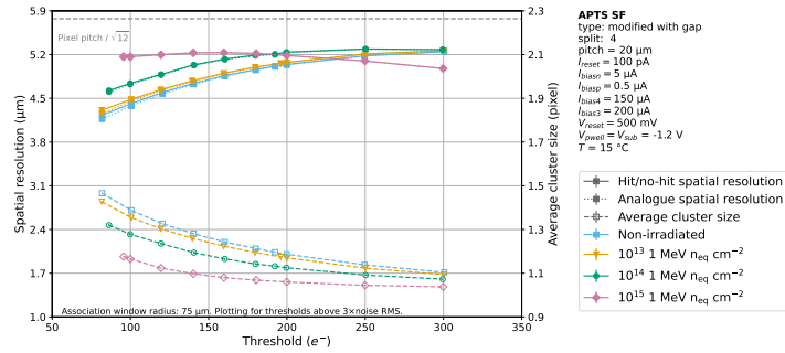
Figure B.44: Resolution comparison between different NIEL irradiation levels as a function of the applied seed threshold. Chiller temperature was 15 \text{ }^\circ\text{C} . APTS with 20 \mu\text{m} pitch, modified with gap, split 4, reference variant, V_{\text{sub}} = -1.2 \text{ V} .
