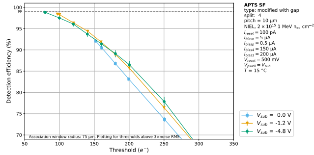
Figure B.36: Efficiency comparison between different substrate reverse biases as a function of the applied seed threshold for a NIEL irradiation level of 2 \times 10^{15} \text{ 1 MeV } n_{\text{eq}} \text{ cm}^{-2} . Chiller temperature was 15 \text{ }^\circ\text{C} . APTS with 10 \text{ }\mu\text{m} pitch, modified with gap, split 4, reference variant, V_{\text{sub}} = -1.2 \text{ V} .
