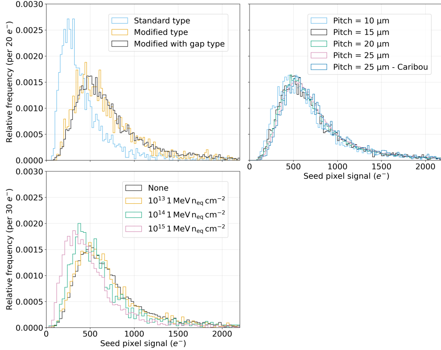
Figure 12: (Top left) Comparison between different designs of the seed pixel signal charge distribution for a pitch of 15\ \mu\text{m} . (Top right) Comparison between different pixel pitch sizes of the seed pixel signal charge distribution for modified with gap sensors. For the Caribou measurement, an I_{\text{bias4}} = 546\ \mu\text{A} has been set. (Bottom) Comparison between different NIEL irradiation doses of the seed pixel signal charge distribution for a modified with gap sensor with a pitch 15\ \mu\text{m} . APTS with split 4, reference variant, V_{\text{sub}} = -1.2\ \text{V} .
