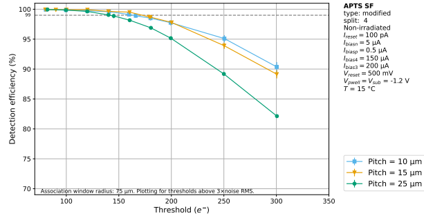
Figure B.30: Efficiency comparison between different pitches as a function of the applied seed threshold. APTS with modified, split 4, reference variant, V_{\text{sub}} = -1.2 \text{ V} .
