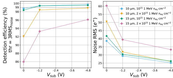
Figure 15: Comparison of efficiency and noise versus substrate reverse bias for different pitches and radiation levels. APTS with split 4, modified with gap, reference variant.
