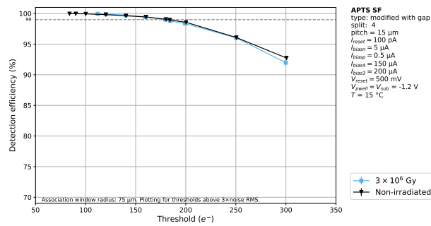
Figure B.34: Efficiency comparison with TID irradiated APTS as a function of the applied seed threshold. Chiller temperature was 15 °C. APTS with 15 μm pitch, modified with gap, split 4, reference variant, V_{sub} = -1.2 \text{ V} .
