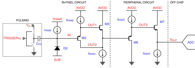
Figure 4: A schematic of the front-end chain of APTS.
