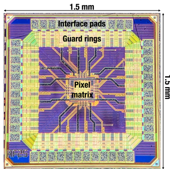
Figure 1: Photo of the APTS chip under a microscope.
