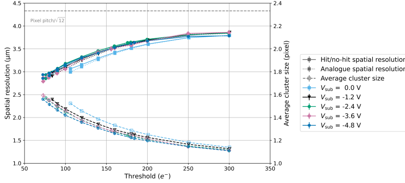
Figure 16: Hit/no-hit resolution (solid lines), analogue resolution (dotted lines) and average cluster size (dashed lines) vs threshold at different V_{\text{sub}} values. The chiller temperature was set to T = 15 °C. APTS with 15 \mu\text{m} pitch, modified with gap, split 4, reference variant.
