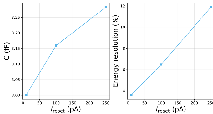
Figure A.18: Capacitance (left) and energy resolution (right) comparison between different I_{\text{reset}} . APTS with 15 \mu\text{m} pitch, modified with gap, split 4, reference variant, V_{\text{sub}} = -1.2 V, standard readout.
