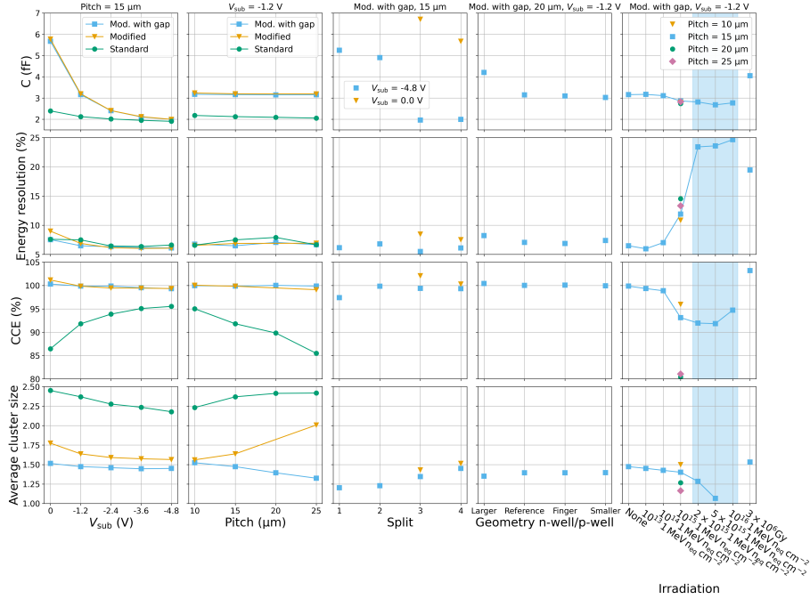
Figure 10: Comparison of the main characteristics extracted from the ^{55}\text{Fe} spectra. The light blue window in the last column refers to the data points acquired with I_{\text{reset}} = 250 pA.
