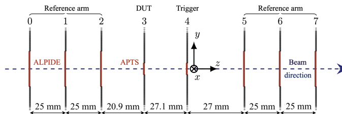
Figure 11: Scheme of the telescope setup used at the SPS test beams. The planes 3 and 4 were made with APTS chips, all others with ALPIDE chips. Not to scale.
