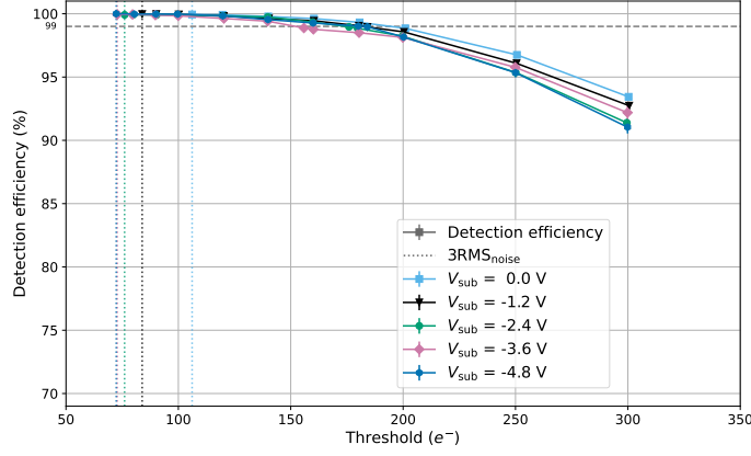
Figure 13: Efficiency comparison between different reverse substrate voltages as a function of the applied seed threshold. The dotted lines indicate the threshold corresponding to 3 times the RMS noise value. APTS with 15 \mu\text{m} pitch, modified with gap, split 4, reference variant.
