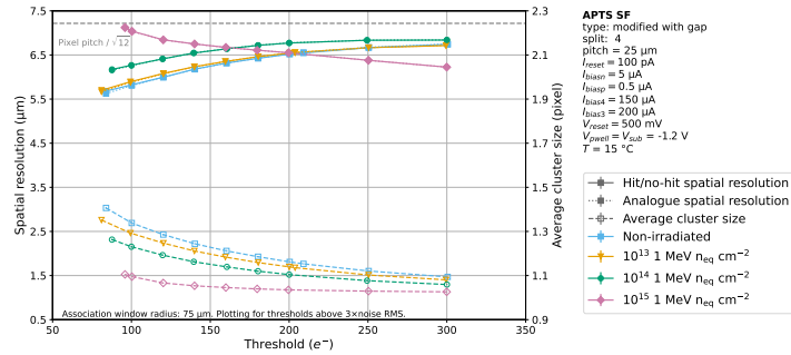
Figure B.45: Resolution comparison between different NIEL irradiation levels as a function of the applied seed threshold. Chiller temperature was 15 °C. APTS with 25 \mu\text{m} pitch, modified with gap, split 4, reference variant, V_{\text{sub}} = -1.2 \text{ V} .
