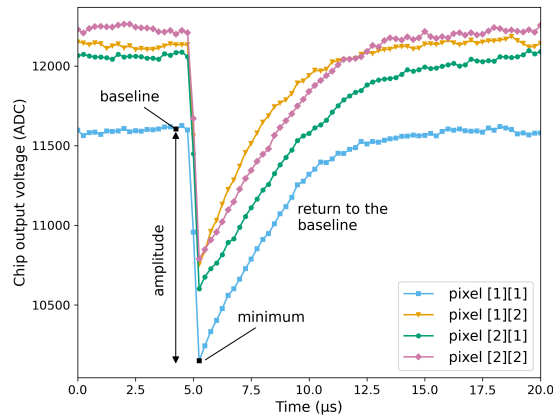
Figure 5: Typical uncalibrated chip output signal from the 4 innermost pixels of an APTS chip pulsed with V_{\text{H}} = 1.2 V. APTS with 15 \mu\text{m} pitch, modified with gap, split 4, reference variant, V_{\text{sub}} = -1.2 V.
