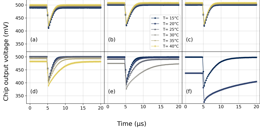
Figure 6: Comparison at different temperatures of the signal waveform pulsed with V_H = 1.2 V, averaged over 1000 events, for chips at different irradiation levels, using an optimized working point with increased I_{\text{reset}} of 250 pA in order to compensate for leakage current: (a) Not irradiated, (b) 10^{13} 1 \text{ MeV n}_{\text{eq}} \text{ cm}^{-2} , (c) 10^{14} 1 \text{ MeV n}_{\text{eq}} \text{ cm}^{-2} , (d) 10^{15} 1 \text{ MeV n}_{\text{eq}} \text{ cm}^{-2} , (e) 2 \times 10^{15} 1 \text{ MeV n}_{\text{eq}} \text{ cm}^{-2} and (f) 10^{16} 1 \text{ MeV n}_{\text{eq}} \text{ cm}^{-2} . APTS with 15 \mu\text{m} pitch, modified with gap, split 4, reference variant, V_{\text{sub}} = -1.2 V.
