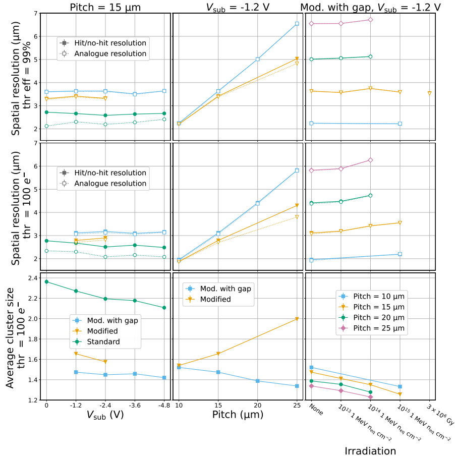
Figure 17: Comparison of the main characteristics extracted from the resolution plots versus threshold. APTS with split 4, reference variant.
