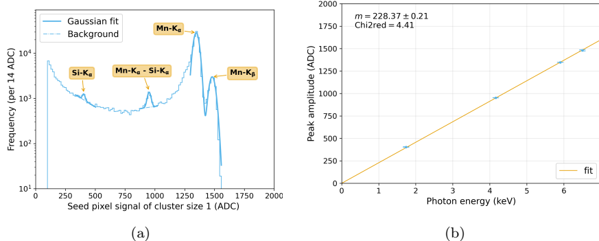
Figure 8: (a) ^{55}\text{Fe} spectrum for events with cluster size 1. The seed distribution is filled with the seed signals of the 4 central pixels of the matrix. (b) Energy calibration was obtained using the peak means from the Gaussian fits on (a). Data are fitted with a linear function, where m is the slope parameter. The errors refer to the ones obtained from the fits. All these measurements were taken at I_{\text{reset}} = 10 pA for a better energy resolution, as explained in Appendix A. APTS with 15\ \mu\text{m} pitch, modified with gap, split 4, reference variant, V_{\text{sub}} = -1.2 V.
