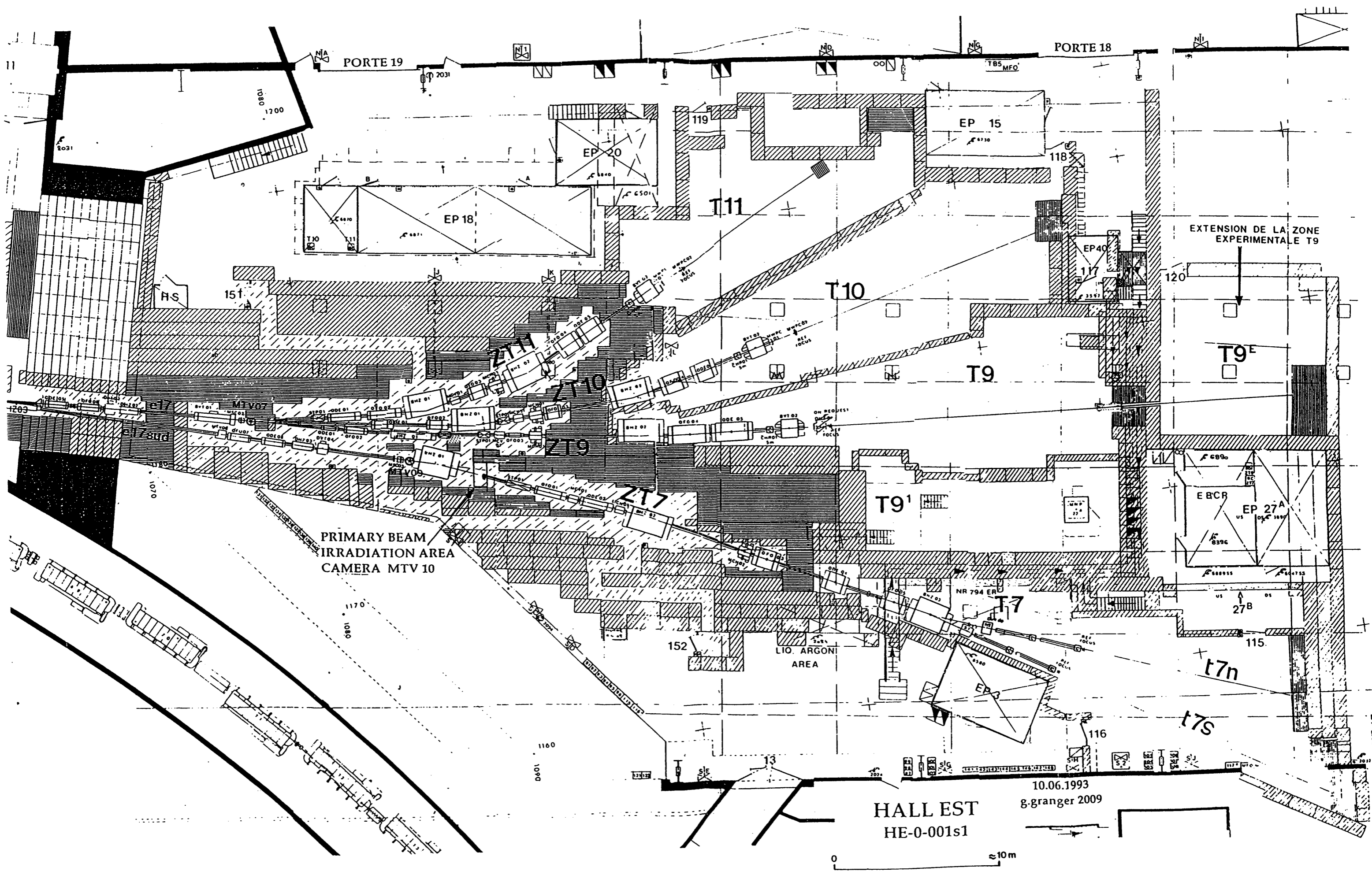
Figure 1 : East Hall floor plan
