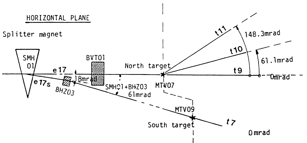
Schematic layout of the secondary beams
