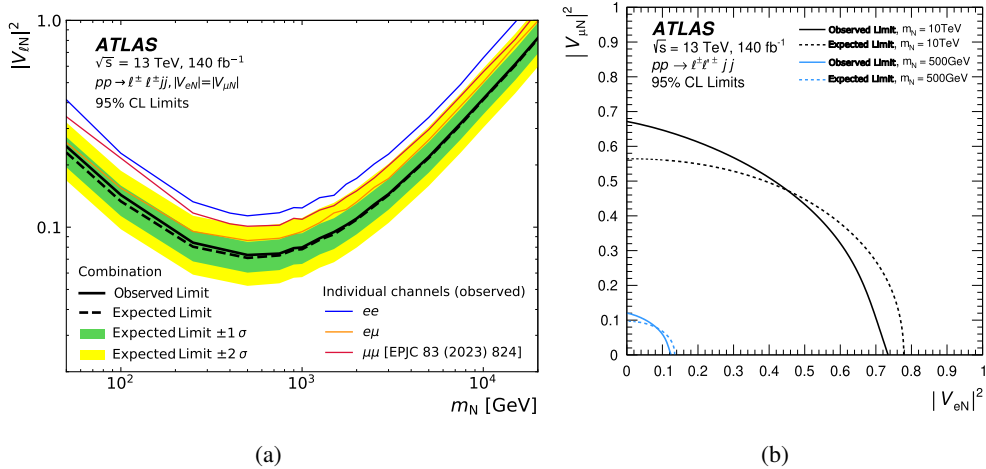
Figure 4: (a) Observed and expected 95% CL upper limits on the heavy Majorana neutrino mixing element |V_{\ell N}|^2 as a function of m_N and (b) two-dimensional observed and expected 95% CL intervals on |V_{eN}|^2 and |V_{\mu N}|^2 for m_N = 500 GeV and 10 TeV in the Phenomenological Type-I Seesaw model. The limits on the |V_{\ell N}|^2 are obtained assuming |V_{\mu N}|^2 = |V_{eN}|^2 . The observed limits on the |V_{\ell N}|^2 obtained separately in the ee , e\mu , and \mu\mu [14] channels are also shown for comparison. The one and two standard deviation bands of the expected limit are indicated in green and yellow, respectively.
