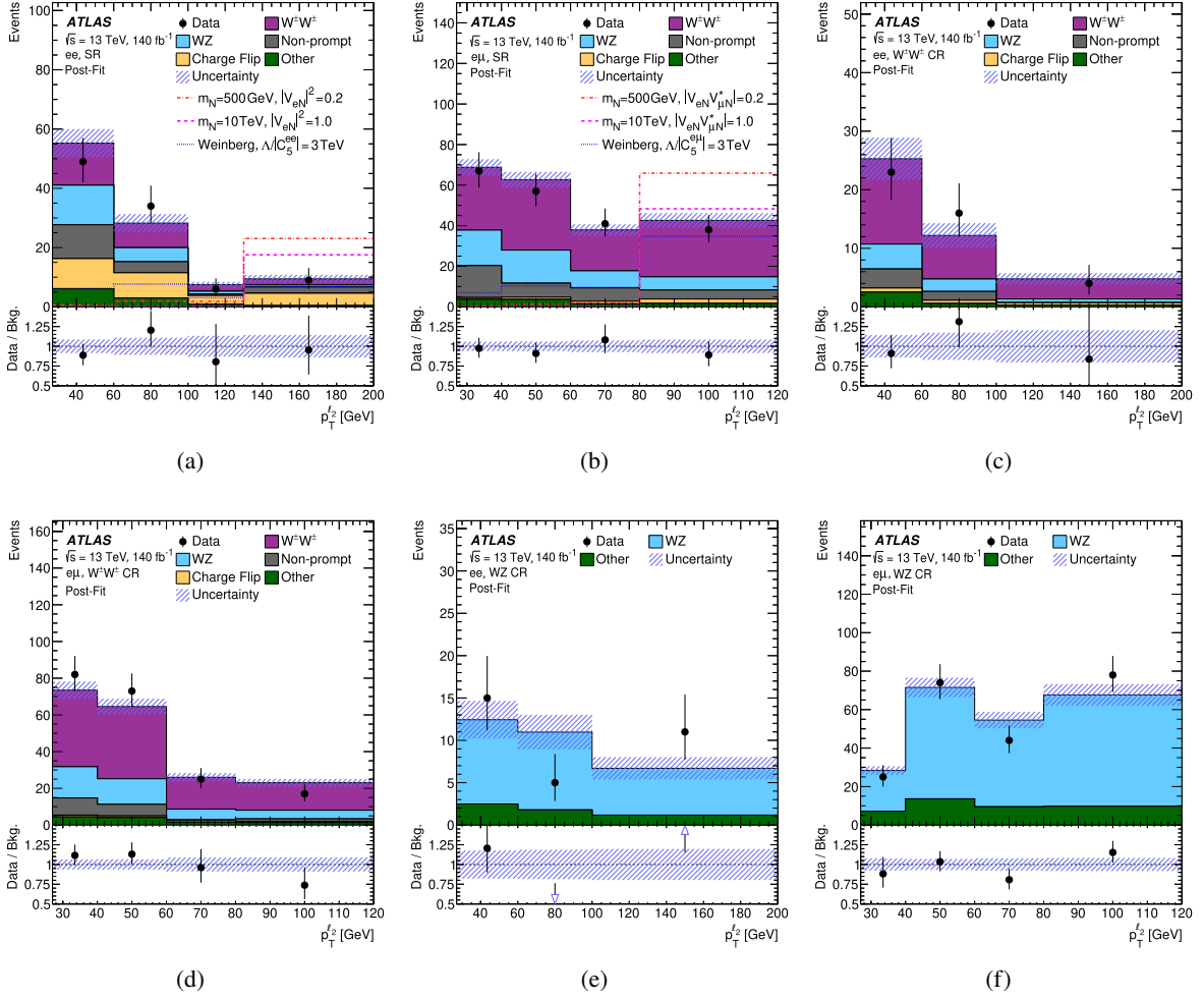
Figure 2: Distributions of the p_T^{\ell_2} in (a) the ee SR, (b) the e\mu SR, (c) the ee same-sign WW CR, (d) the e\mu same-sign WW CR, (e) the ee WZ CR, and (f) the e\mu WZ CR. The predicted yields are shown with their best fit normalization and shape from the fit for the SM background-only fit hypothesis. The shaded area surrounding the background expectation represents the total uncertainties in the predicted yields. The ratios of the observed yields to the total SM predictions are shown by the points in the bottom panels. ‘Other’ includes contributions mainly from the \ell\gamma jj , ZZ and tZq background processes. Benchmark signal predictions are shown as hatched lines. The last bin includes the overflow.
