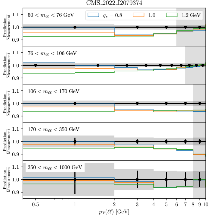
Figure 7: Drell-Yan cross section ratios of MCatNLO+CAS3 predictions for different q_s values over CMS measurement [17] as a function of p_T(\ell\ell) for different m_{D\Upsilon} regions. Only the lowest p_T(\ell\ell) values are shown. The points error bar show the statistical uncertainties and the gray bands the total experimental uncertainties. The gray area at the highest p_T(\ell\ell) values show the maximal values included in the fit described in section 3.2.
