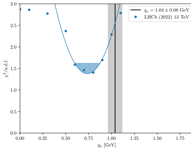
Figure 10: The reduced \chi^2/\text{n.d.f} distribution as a function of q_s summed over all rapidity regions obtained from a comparison of the MCatNLO+CAS3 prediction with the measurement by LHCb [58]. The shaded area corresponds to \chi^2 + 1 . The best fit value is q_s = 0.74 \pm 0.15 GeV. The value of q_s = 1.04 \pm 0.08 GeV as obtained from the measurements in Ref. [17] is indicated by a black vertical line.
