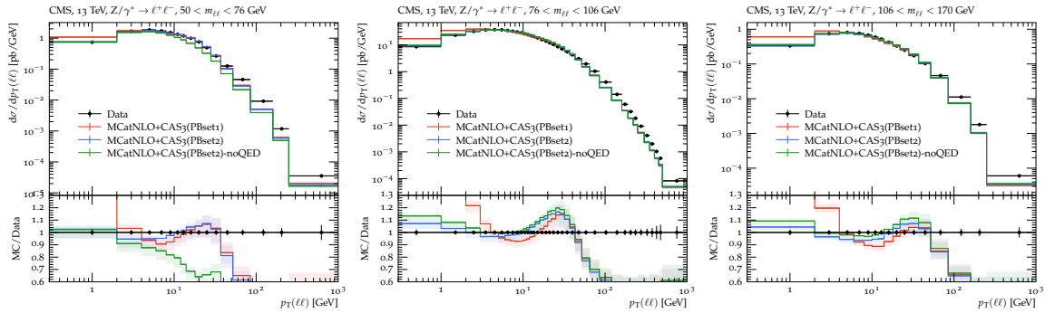
Figure 6: The p_T(\ell\ell) dependent DY cross section for different m_{\text{DY}} regions as measured by CMS [17] compared to MCatNLO+CAS3 predictions based on PB-NLO-2018 Set 1 (red curve) and Set 2 (blue curve). Also shown are predictions without the inclusion of final state QED radiation from the leptons (green curve). The band shows the 7-point variation of the renormalization and factorization scales.
