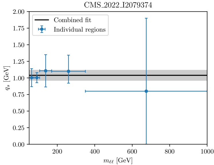
Figure 9: The values of q_s in each m_{\text{DY}} -bin as obtained from Ref. [17]. Indicated is also the combined fit value of q_s .
