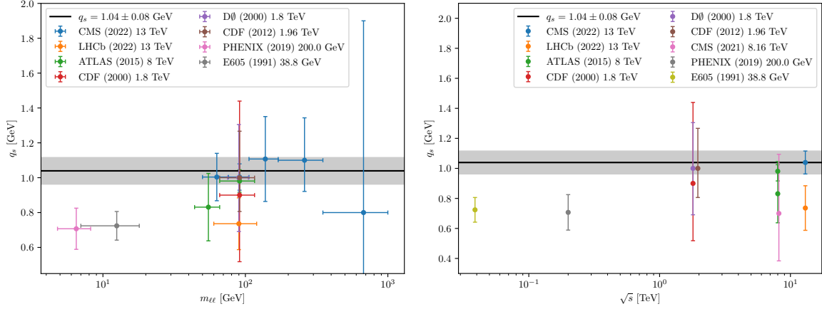
Figure 13: Left : the value of q_s as a function of the DY-mass as obtained from the measurements in Refs. [17,58,61–67]. Right : same as a function of \sqrt{s} . The value of q_s = 1.04 \pm 0.08 GeV as obtained from the measurements in Ref. [17] is indicated.
