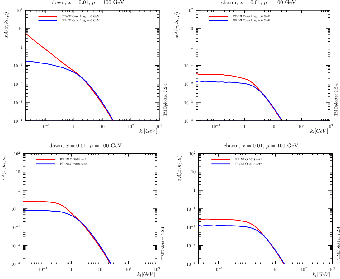
Figure 3: TMD parton density distributions for down and charm quarks of the published PB-NLO-2018 Set1 (red curve) and PB-NLO-2018 Set2 (blue curve) [20] as a function of k_T at \mu = 100 GeV and x = 0.01 . In the upper row are shown distributions when no intrinsic- k_T distribution is included ( q_s = 0.00001 GeV), and the lower row shows the default distributions with q_s = 0.5 GeV.
