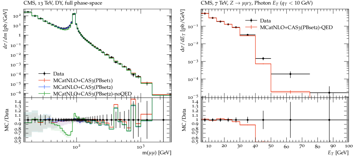
Figure 5: Left: The mass distribution of DY lepton pairs at 13 TeV [51] compared to predictions of MCatNLO+CAS3 with PB-NLO-2018 Set1 (red curve), PB-NLO-2018 Set2 (blue curve) and without QED corrections (green curve). Right: The spectrum of photons transverse momentum in Z \rightarrow \mu^+ \mu^- \gamma at 7 TeV [55] compared to MCatNLO+CAS3 PB-NLO-2018 Set2 including QED radiation for a transverse momentum of the DY pair p_T(\ell\ell) < 10 GeV. The bands show the scale uncertainty.
