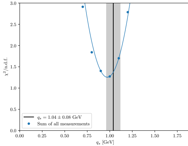
Figure 12: The reduced \chi^2/\text{n.d.f.} distribution (n.d.f. = 81) as a function of q_s obtained from a comparison of the MCatNLO+CAS3 PB-NLO-2018 Set2 prediction with the measurement of Refs. [17,58,61–67]. The minimum of global DY data fit is close to q_s = 1 GeV and consistent with the CMS measurement [17] shown separately by a black line.
