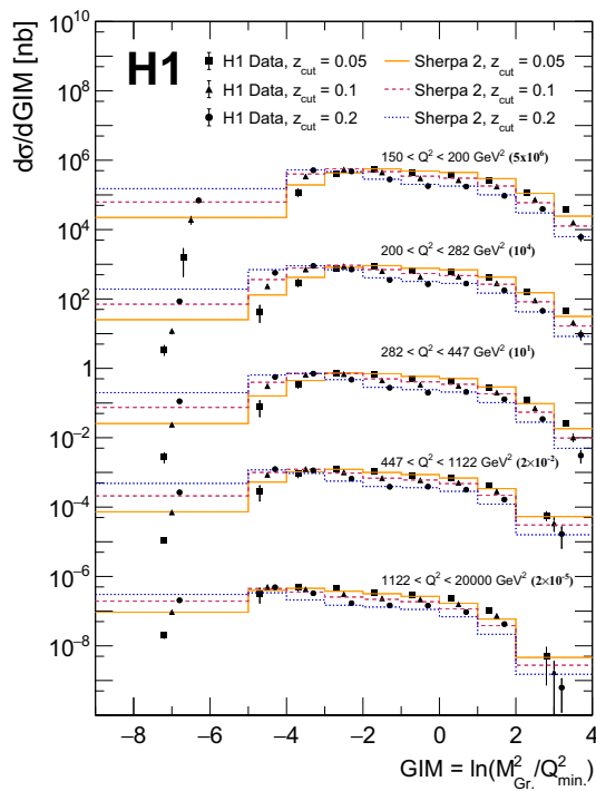
Fig. 6 Double-differential groomed invariant mass distributions for z_{\text{cut}} = 0.05, 0.1, \text{ and } 0.2 , for five bins in Q^2 . The value of Q_{\text{min}}^2 is taken to be the lowest value of Q^2 in the bin, e.g. 1122 \text{ GeV}^2 for the highest Q^2 bin. Uncertainty bars on the data show the quadrature sum of the statistical and systematic uncertainties. The data points are horizontally offset from the bin center for visibility. The lines represent predictions from Sherpa 2 using the cluster hadronization model. The five distributions at different values of Q^2 are vertically offset by the factor given in parentheses
