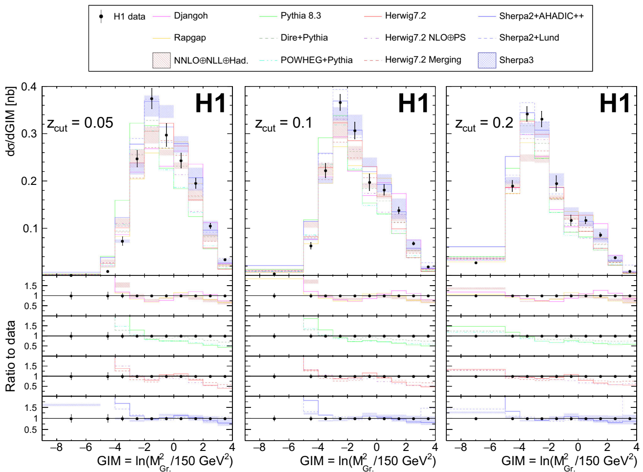
Fig. 2 Differential cross section of groomed invariant mass GIM = \ln(M_{Gr}^2/150 \text{ GeV}^2) in ep DIS at \sqrt{s} = 319 \text{ GeV} , for z_{cut} = 0.05, 0.1 and, 0.2 . The value of Q_{min}^2 is set to 150 \text{ GeV}^2 . The phase space is restricted to Q^2 > 150 \text{ GeV}^2 and 0.2 < y < 0.7 . Uncertainty bars on
