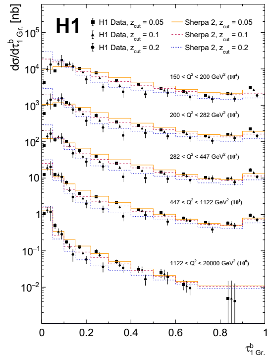
Fig. 7 Double-differential \tau_{1\text{Gr}}^b cross section for z_{\text{cut}} = 0.05, 0.1, \text{ and } 0.2 , presented in five bins in Q^2 . Further details are given in the caption of Fig. 6
