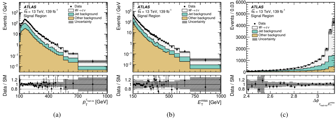
Figure 4: Distributions of (a) the transverse momentum of the \tau_{\text{had-vis}} candidate, p_{\text{T}}^{\tau_{\text{had-vis}}} , (b) the missing transverse momentum in the event, E_{\text{T}}^{\text{miss}} , and (c) the azimuthal angle between the \tau_{\text{had-vis}} candidate and the missing transverse momentum, \Delta\phi_{\tau_{\text{had-vis}}, E_{\text{T}}^{\text{miss}}} , in the signal region. The uncertainty band (hatched) shows the total statistical and systematic uncertainty.
