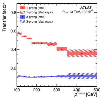
Figure 1: Transfer factors used in the jet-background estimation as a function of p_T^{\text{had-vis}} , for 1-prong (upward triangles) and 3-prong (downward triangles) \tau -lepton decays. The uncertainty due to the limited number of events in CR2 and CR3 is shown as solid filled areas while the hatched areas indicates the total statistical and systematic uncertainties.
