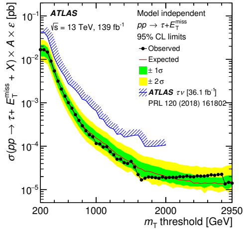
Figure 8: Model-independent 95% CL upper limits on the visible \tau + E_{\text{T}}^{\text{miss}} cross-section as a function of the transverse mass thresholds, m_{\text{T}}^{\text{thresh}} . The blue hatched line shows the observed 95% CL upper limits on the visible \tau + E_{\text{T}}^{\text{miss}} cross-section of the previous ATLAS \tau\nu [10] search. The steps in the observed upper limit at m_{\text{T}}^{\text{thresh}} of 1.6 and 2.85 TeV result of the discrete nature of the data and that the highest m_{\text{T}} event in data appeared with m_{\text{T}} = 2.83 \text{ TeV} .
