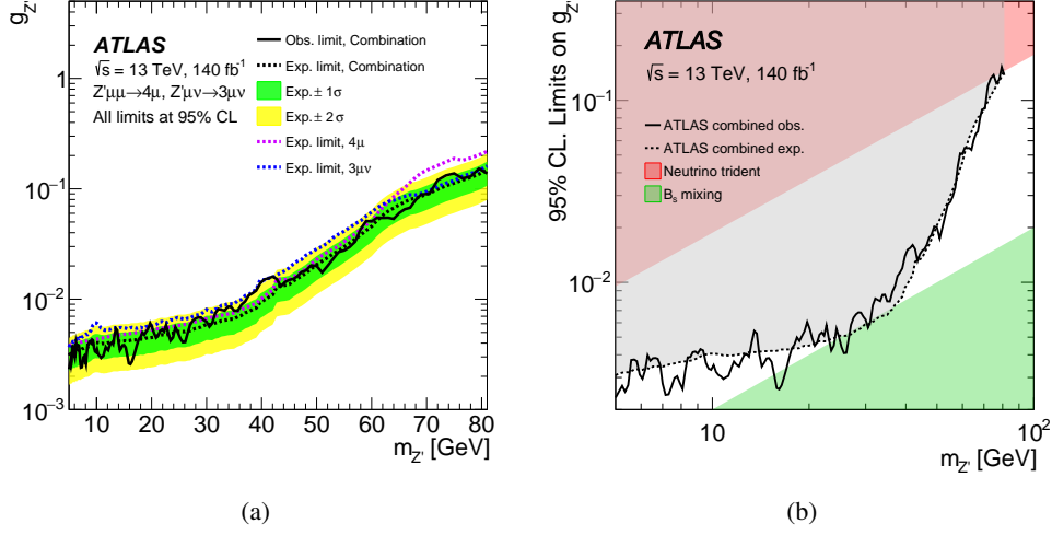
Figure 4: Results from the statistical combination of the 3 \mu and 4 \mu channels: (a) observed and expected 95% CL upper limits on g as a function of m_{Z'} , (b) exclusion contour of g compared with the limits inferred from the neutrino-trident (red) and the B_s mixing (green) experimental results [19].
