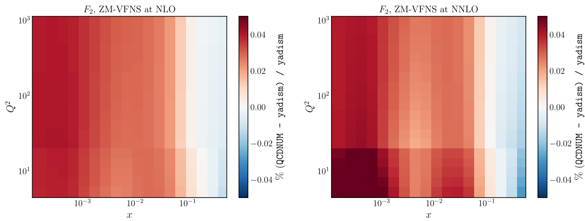
Fig. 1 Relative difference between yadism and QCDNUM for the structure function F_2 using ZM-VFNS as function of x and Q^2 at NLO (left) and NNLO (right) accuracy
