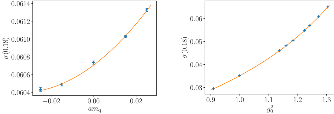
Figure 1: Quadratic fit of \sigma(0.18) vs. am_q for L/a = 24 , \beta = 4.7141 (left), and nine-point fit with n_g = 5 of \sigma(0.18) vs. g_0^2 for L/a = 24 and 4.6 \leq \beta \leq 6.6 (cf. table 5) (right).
