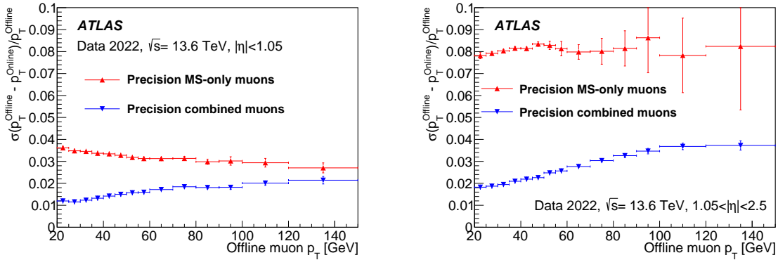
Figure 30. Width of the residuals for p_T as a function of the offline muon p_T for the precision MS-only and combined algorithms in (left) the barrel and (right) the endcaps. Only statistical uncertainties are shown.
