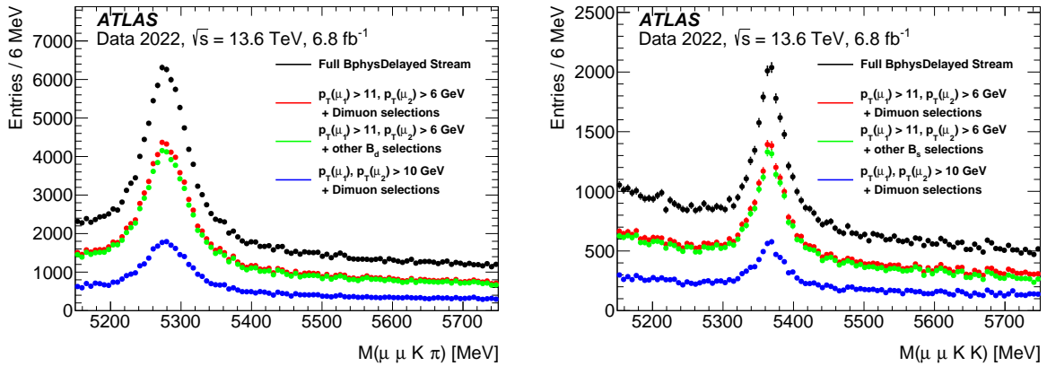
Figure 50: To validate the selection of the b\text{BmumuX} the mass spectra of the selected (left) B_d \rightarrow J/\psi K^* and (right) B_s \rightarrow J/\psi \phi events from the BLS Delayed stream are plotted along with the spectra for a variety of bJ\psi\text{simumu} and b\text{BmumuX} trigger decisions. Only statistical uncertainties are shown.
