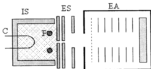
Figure 1: Schematic of the experimental arrangement. A multicusp ion source (IS) with filter magnets (F) is used for filament-driven plasma generation (C). Attached to the source body is the triode extraction system (ES). The high-voltage, retarding-field analyzer (EA) is placed 50 cm behind the extraction system. It consists of an electron suppression grid at the entrance, a column of electrodes for deceleration and an analyzer plate for collection of the ions.
