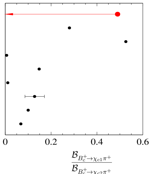
Figure 5. Comparison of upper limit on the branching fraction ratio between B_c^+ \rightarrow \chi_{c1}\pi^+ and B_c^+ \rightarrow \chi_{c2}\pi^+ decays set in this analysis with theoretical predictions.
