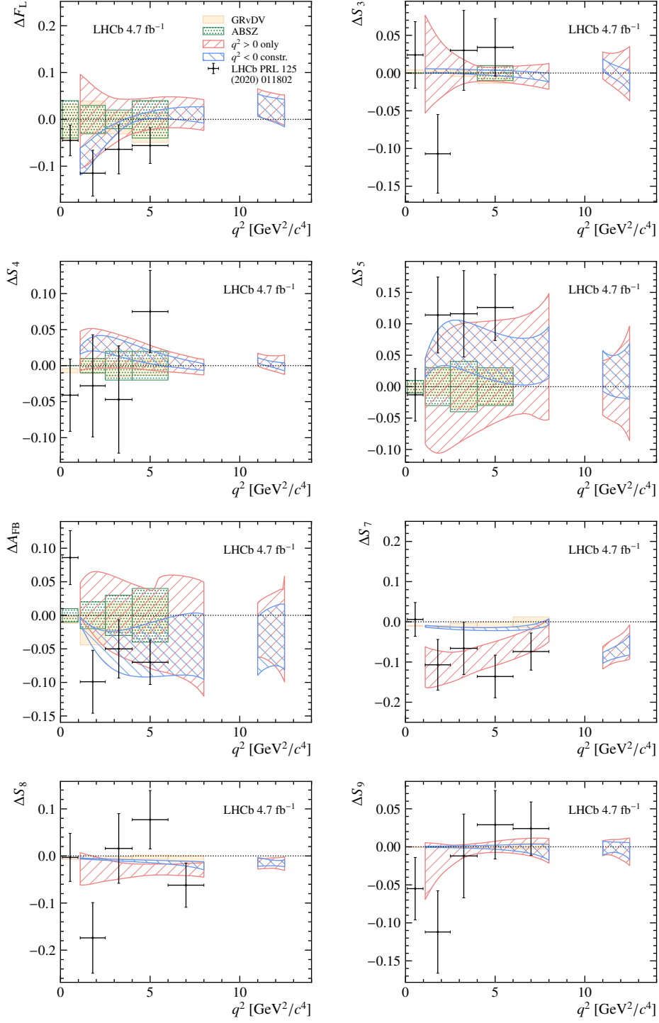
Figure 5: Non-local contributions to the angular observables (S-basis) obtained from data fits with (blue) and without (red) constraints from q^2 < 0 . The shaded regions are shown at 68% confidence level. When available, the difference between the LHCb binned angular analysis [10] and SM central-value from Refs. [23, 70] is overlaid for reference (black dots), together with the uncertainty on the SM prediction (green) and difference between the SM predictions from Refs. [16, 25, 31] with respect to Refs. [23, 70] (yellow).
