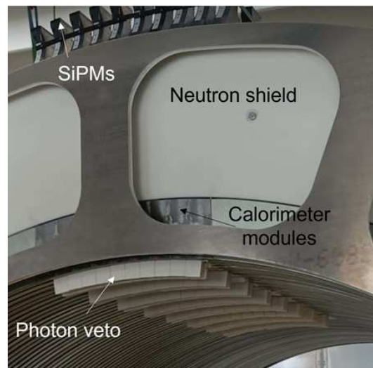
Figure 2. View of the ENUBET demonstrator tested at CERN in 2022. The prototype corresponds to a fraction of the instrumented decay tunnel with a curvature radius of 1 m [9]. It comprises a scintillator-based photon veto and a modular calorimeter. The scintillation light produced in the calorimeter and in the veto is brought to the outer part of the detector by means of wavelength-shifting fibers and read out by SiPMs. SiPMs are protected from fast neutrons by a borated plastic shield.
