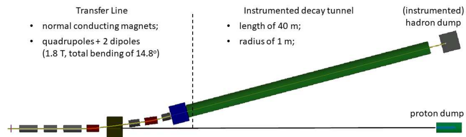
Figure 1. Layout of the ENUBET monitored neutrino beam at CERN. Protons impinging on the target produce secondaries that are sign- and momentum-selected using a static (i.e., hornless) transfer line. They are steered to the decay tunnel. Particles impinging on the tunnel wall are detected by the instrumentation (segmented calorimeters) installed in the tunnel. Undecayed secondaries are stopped by the hadron dump, while protons that did not interact with the target are stopped by the proton dump.
