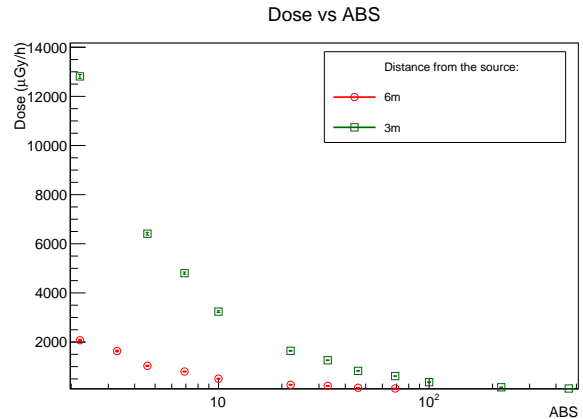
Fig. 2 Dose measured in the GIF++, at 3 and 6 m from the ^{137}\text{Cs} source, as a function of the ABS
