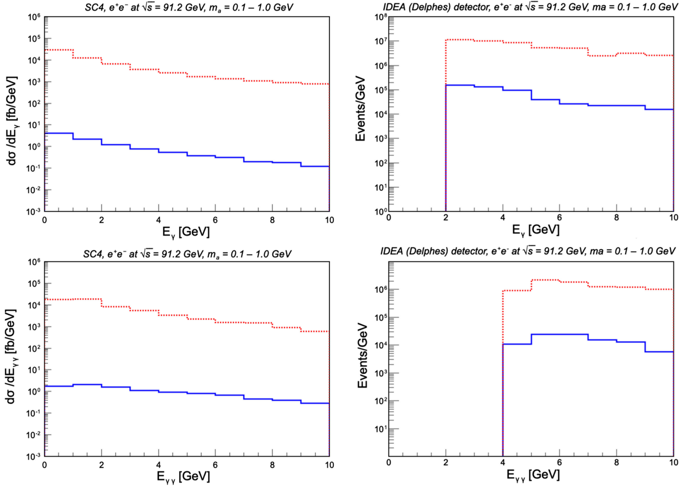
FIG. 4. Distributions of the energy of single- \gamma ( E_\gamma ) and \gamma\gamma pairs ( E_{\gamma\gamma} ) for simulated ALPs in the mass range m_a = 0.1-1.0 GeV and coupling g_{a\gamma\gamma} = 0.1 \text{ TeV}^{-1} (blue histogram) and for the LbL continuum (dashed red histogram) in e^+e^- collisions at FCC-ee at \sqrt{s} = 91.2 GeV. The left (right) plots show generator-level (IDEA reconstruction-level) results.
