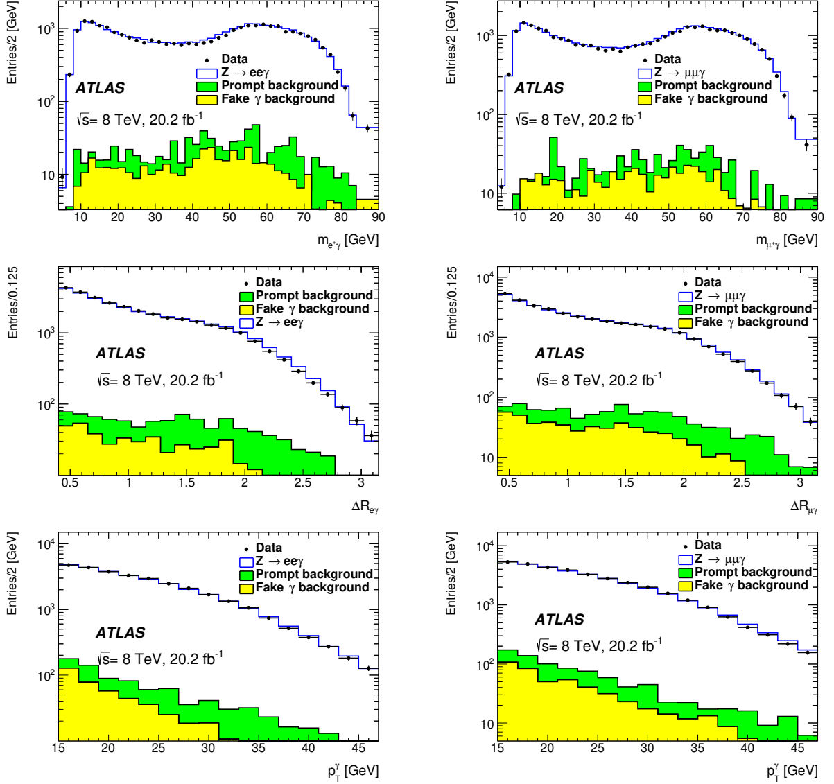
Figure 5: For electrons (left) and muons (right), measured differential rates for m_{l\gamma} (top), \Delta R_{l\gamma} (middle), and p_T^\gamma (bottom). The data are shown compared to the sum of the expected contributions from the Z \rightarrow ll\gamma signal, as predicted from Powheg+Pythia8+Photos, and of the prompt and fake \gamma backgrounds.
