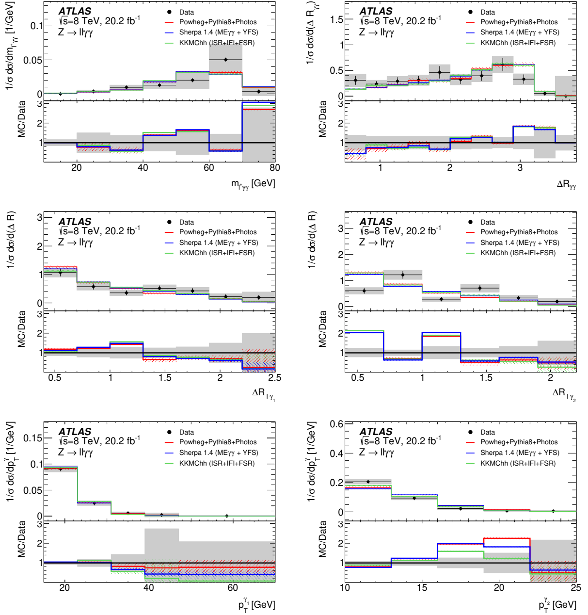
Figure 10: For all selected Z \rightarrow ll\gamma\gamma candidates, unfolded normalised distributions of m_{l+\gamma\gamma} (top left), of \Delta R_{\gamma\gamma} (top right), of the angular distance between the first (middle left) and second (middle right) photon and the closest lepton, and of the transverse momentum spectrum of the two photons (bottom). The unfolded data are compared to predictions from Powheg+Pythia8+Photos, Sherpa 1.4 ME_{\gamma\gamma} , and KKMChh. The results are shown for bare leptons, and electrons and muons have been combined. The gray band represents the total data uncertainties and the dashed lines around the predictions represent their statistical uncertainties, which are dominant, for the predictions.
