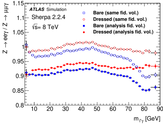
Figure 3: Predicted ratios of expected differential cross-sections for the invariant mass, m_{l+\gamma} , of the positively charged lepton and the photon (left) and of the angular separation, \Delta R_{l\gamma} , between the photon and the closer of the two leptons (right) for electrons compared to muons. The ratios are shown for the bare and dressed lepton definitions described in the text. The predictions are obtained from a high-statistics inclusive Z-boson sample using Sherpa 2.2.4 and are shown for events containing two high- p_T leptons and one high- p_T photon satisfying the fiducial volume selections described in Table 2 in Section 6 (full symbols). Since most of the difference between electrons and muons observed in this case for the bulk of the distributions is due to the higher acceptance in \eta for the muons, the electron to muon ratios are also shown in the case of identical fiducial selections for both charged leptons (open symbols).
