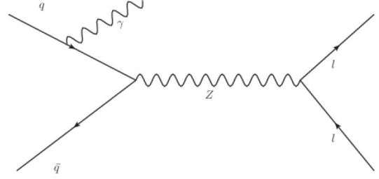
Figure 2: Example of q\bar{q} \rightarrow Z \rightarrow ll\gamma initial-state QED radiation diagram.
