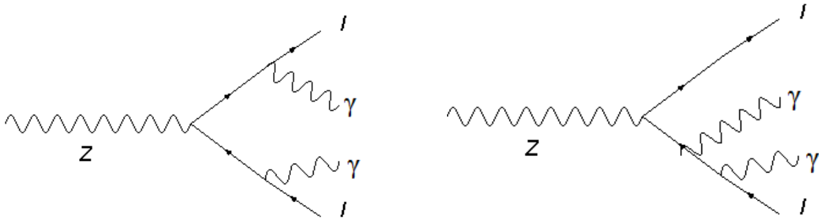
Figure 8: Examples of Z \rightarrow ll\gamma\gamma final-state radiation diagrams.
