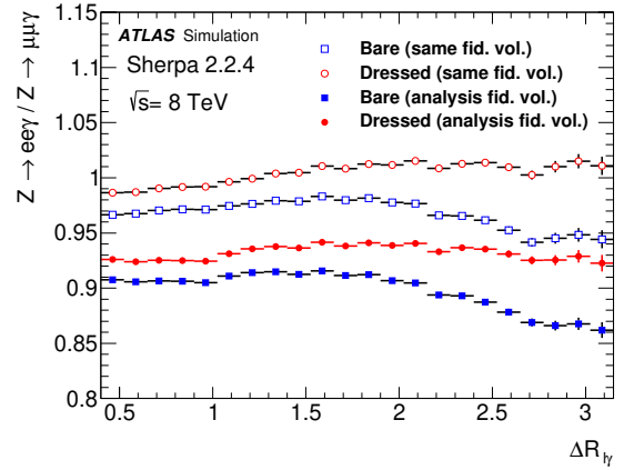
Figure 3: Predicted ratios of expected differential cross-sections for the invariant mass, m_{l+\gamma} , of the positively charged lepton and the photon (left) and of the angular separation, \Delta R_{l\gamma} , between the photon and the closer of the two leptons (right) for electrons compared to muons. The ratios are shown for the bare and dressed lepton definitions described in the text. The predictions are obtained from a high-statistics inclusive Z-boson sample using Sherpa 2.2.4 and are shown for events containing two high- p_T leptons and one high- p_T photon satisfying the fiducial volume selections described in Table 2 in Section 6 (full symbols). Since most of the difference between electrons and muons observed in this case for the bulk of the distributions is due to the higher acceptance in \eta for the muons, the electron to muon ratios are also shown in the case of identical fiducial selections for both charged leptons (open symbols).
