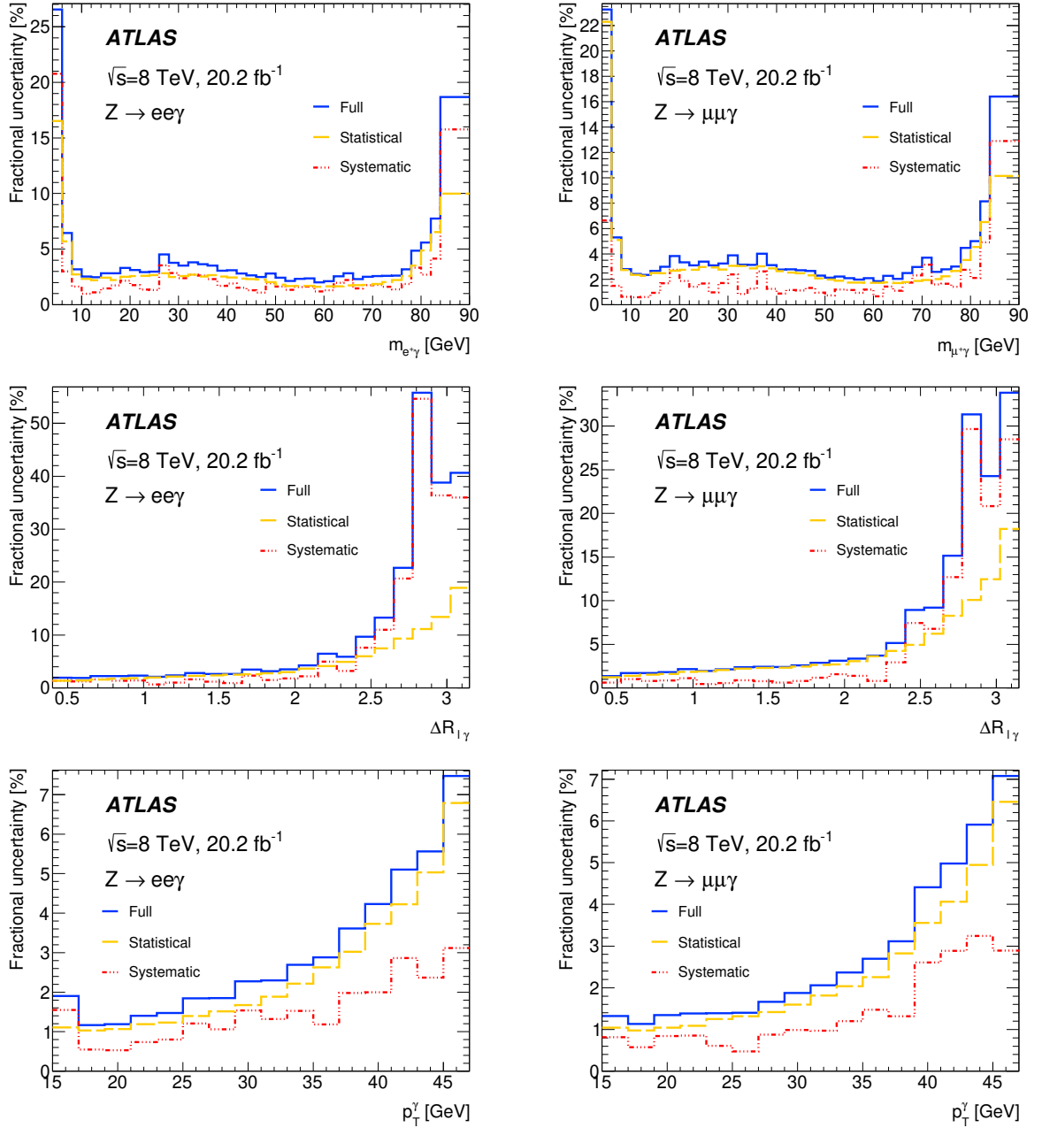
Figure 6: Breakdown of relative uncertainties for the normalised unfolded differential cross-sections as a function of the observables of interest, m_{l+\gamma} (top), \Delta R_{l\gamma} (middle), and p_T^\gamma (bottom), shown separately for the Z \rightarrow ee\gamma (left) and Z \rightarrow \mu\mu\gamma (right) channels.
