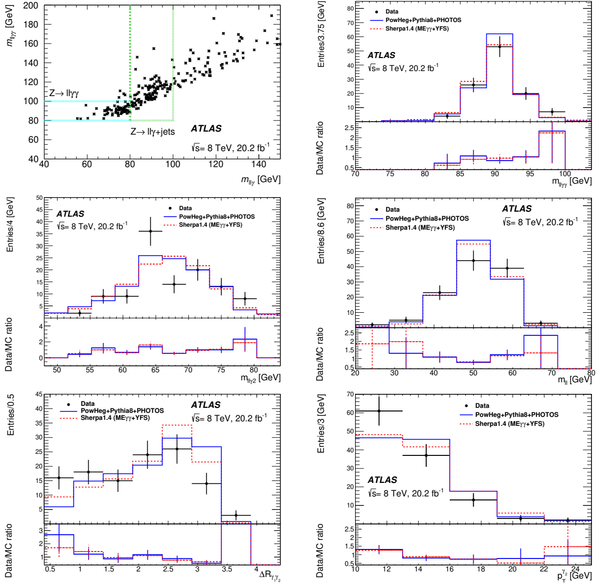
Figure 9: For all selected Z \rightarrow ll\gamma\gamma candidates before applying any selection on the invariant mass of the two leptons and each photon described in the text, distribution of invariant mass of the two leptons and the two photons, m_{ll\gamma\gamma} versus the invariant mass of the two leptons and of the highest p_T photon, m_{ll\gamma} (top left). The horizontal dashed (blue) rectangle indicates the region where the Z \rightarrow ll\gamma\gamma signal is expected and the vertical dashed (green) rectangle indicates the region dominated by background from Z \rightarrow ll\gamma events accompanied by one or more jets. Also shown after all selection requirements are the distributions of the total invariant mass (top right), of the invariant mass of the two leptons and the second photon, of the dilepton mass, of the angular distance between the two photons, and of the transverse momentum of the second photon. The data are compared to predictions from Powheg+Pythia8+Photos and Sherpa 1.4 ME_{\gamma\gamma} , normalised both to the data. The results are shown for bare leptons, and electrons and muons have been combined. The uncertainties shown are statistical.
