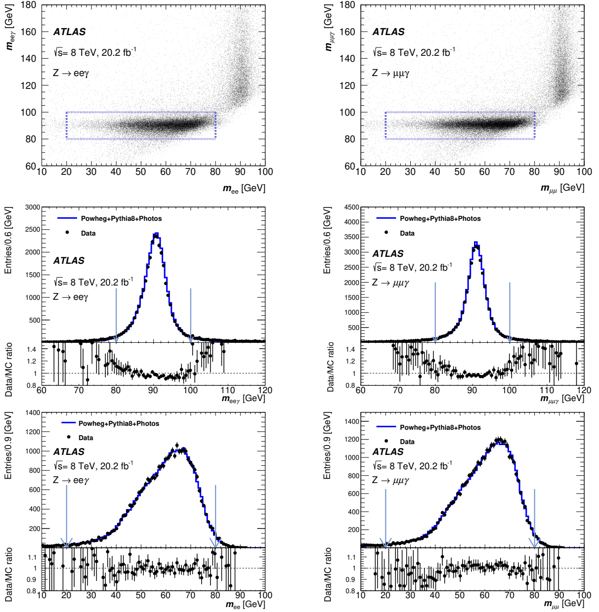
Figure 4: For Z \rightarrow ee\gamma (left) and Z \rightarrow \mu\mu\gamma (right) decay candidates in data, distribution of the three-body invariant mass, m_{ll\gamma} , versus the dilepton mass, m_{ll} . The dashed lines indicate the selection criteria applied in the analysis to these two reconstructed invariant masses. These criteria minimise in particular the background from Z bosons produced in association with jets in which one jet is misidentified as a photon. Also shown are the projections of these figures onto the vertical (middle plot with only the selection on m_{ll} applied) and horizontal (bottom plot with only the selection on m_{ll\gamma} applied) axes with the corresponding vertical lines indicating the selection cuts described above. The curves show the signal predictions from the nominal Powheg+Pythia8+Photos MC normalised to the data.
