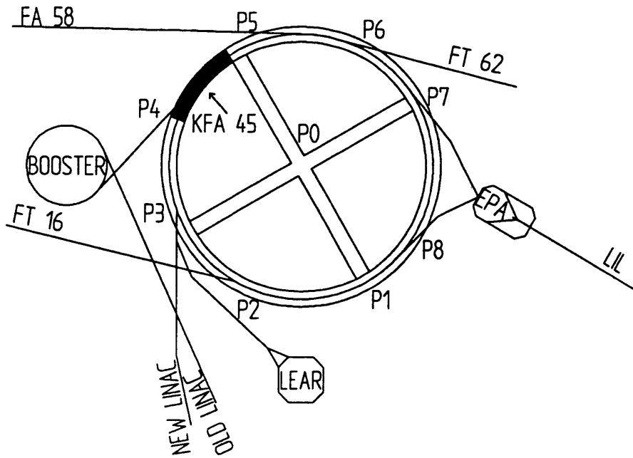
Figure 2a : Localization of the kickers in the PS ring
