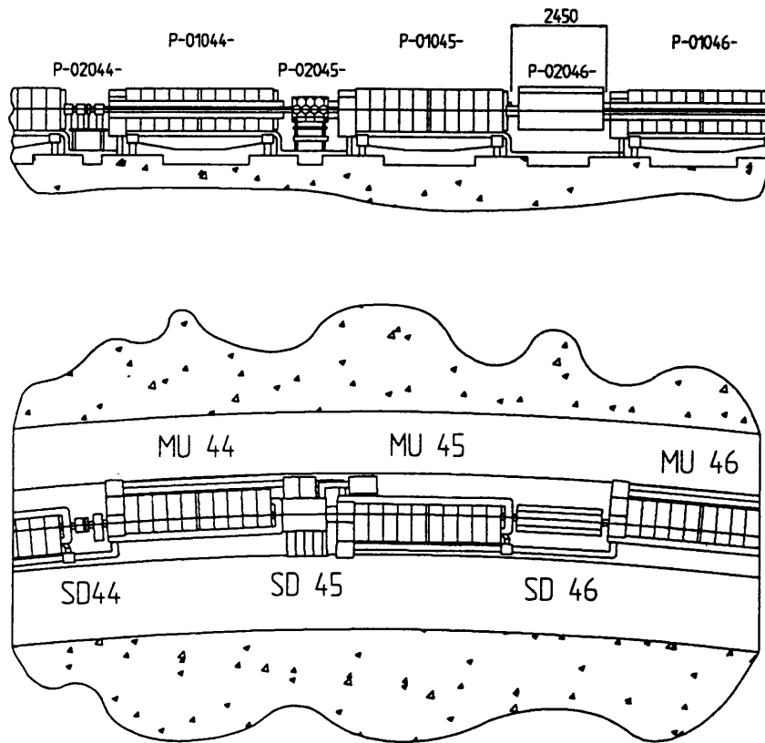
Figure 2a : Localization of the kickers in the PS ring
