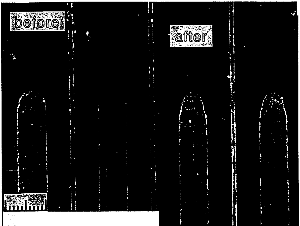
Figure 2: Ends of cathodes before and after discharge (scale = 100 \mu\text{m} ).
