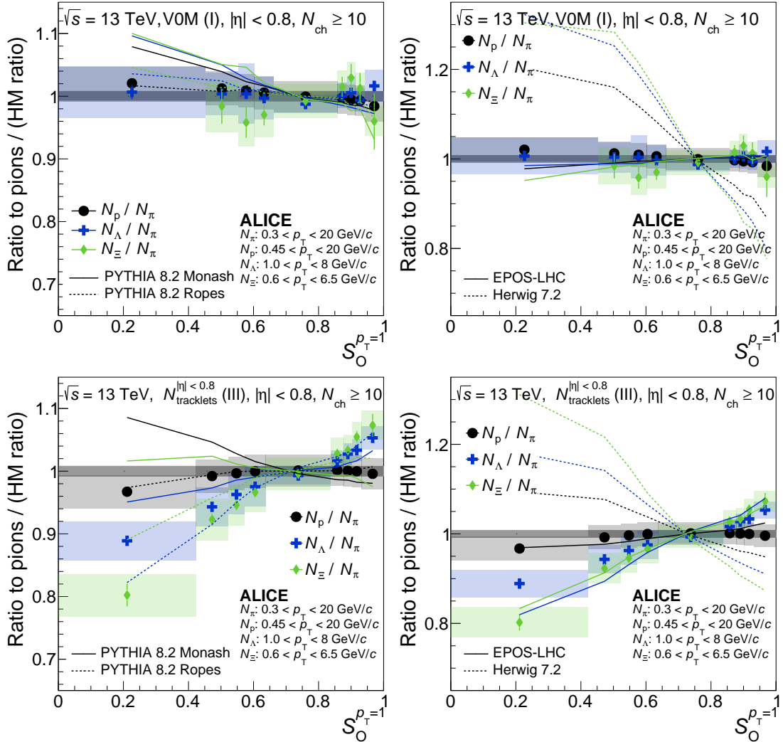
Figure 18: The double ratios of integrated yield as a function of S_O^{p_T=1} are presented for VOM 0–1% (upper) and N_{tracklets}^{|\eta| < 0.8} 0–10% (lower). Left and right panels show the same data points, but with different model predictions. Statistical and total systematic uncertainties are shown by bars and boxes, respectively. The curves represent different model predictions of the same measurement.
