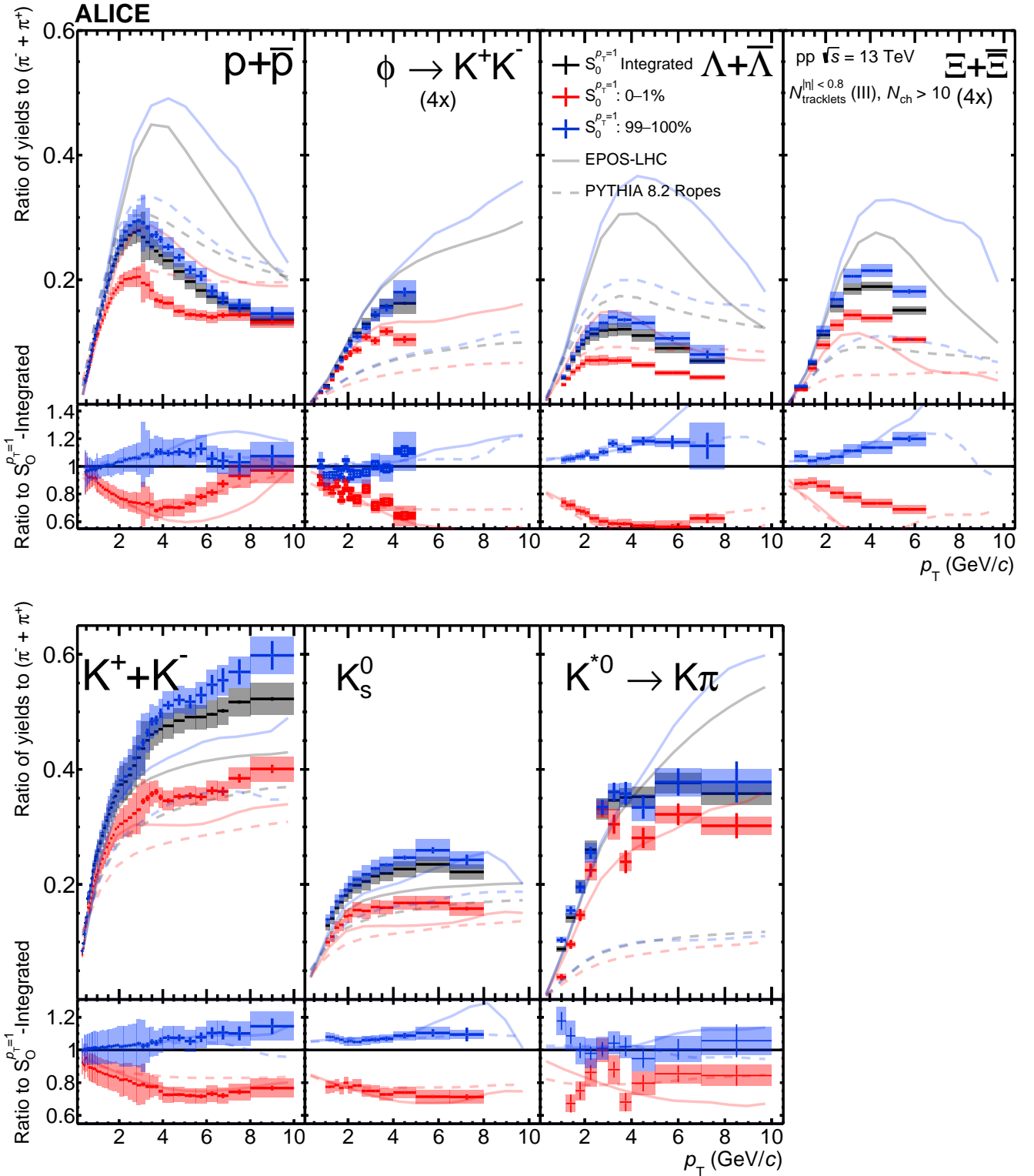
Figure 16: Top panels show hadron-to- \pi ratios for 0–1% S_0^{p_T=1} classes selected for the 0–10% N_{\text{tracklets}}^{|\eta| < 0.8} multiplicity events. Bottom panels present the hadron-to- \pi double-ratios of S_0^{p_T=1} classes relative to S_0^{p_T=1} integrated high-multiplicity events. Statistical and systematic uncertainties are shown by bars and boxes, respectively. Experimental results are compared with predictions from EPOS-LHC and PYTHIA 8.2 Rope hadronization framework.
