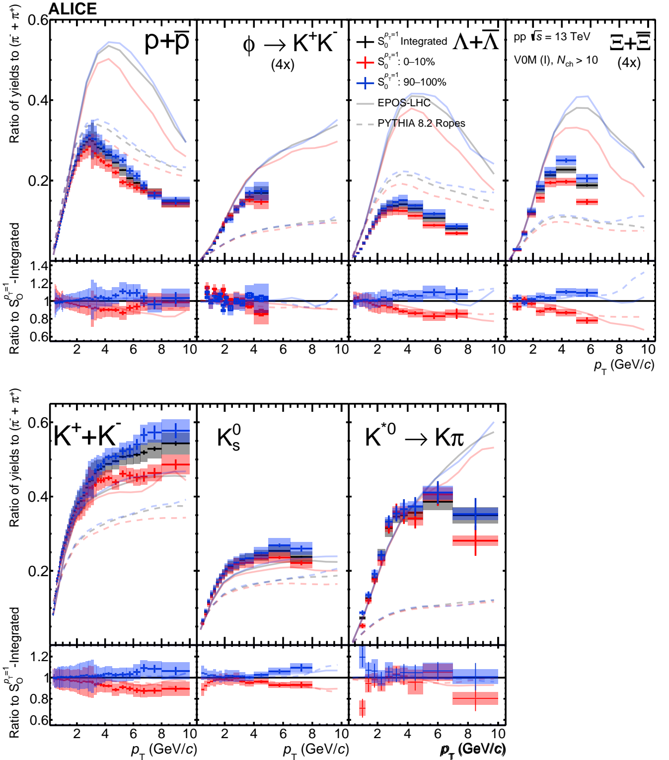
Figure 17: Top panels show hadron-to- \pi ratios for 0–10% S_0^{p_T=1} classes selected for the 0–1% V0M multiplicity events. Bottom panels present the hadron-to- \pi double-ratios of S_0^{p_T=1} classes relative to S_0^{p_T=1} integrated high-multiplicity events. Statistical and systematic uncertainties are shown by bars and boxes, respectively. Experimental results are compared with predictions from EPOS-LHC and PYTHIA 8.2 Rope hadronization framework.
