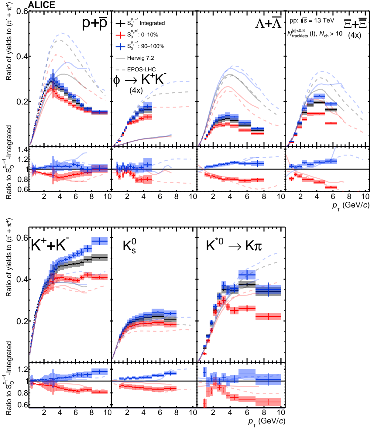
Figure 8: Top panels show hadron-to- \pi ratios for 0–10% S_0^{p_T=1} classes selected for the 0–1% N_{\text{tracklets}}^{|\eta| < 0.8} multiplicity events. Figure 7 and Fig. 8 both contain the same experimental data, but the vertical ranges are modified to accommodate the model predictions. Bottom panels present the hadron-to- \pi double ratios of S_0^{p_T=1} classes relative to S_0^{p_T=1} integrated high-multiplicity events. Statistical and systematic uncertainties are shown by bars and boxes, respectively. Experimental results are compared with predictions from Herwig 7.2 and EPOS-LHC. The fluctuations present in the Herwig 7.2 predictions are due to statistical limitations.
