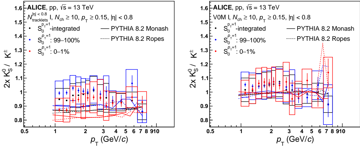
Figure 12: The neutral-to-charged K_S^0/K ratios as a function of different multiplicity estimators and S_O^{p_T=1} . Statistical and total systematic uncertainties are shown by bars and boxes, respectively. The curves represent PYTHIA 8.2 model predictions of the same measurement.
