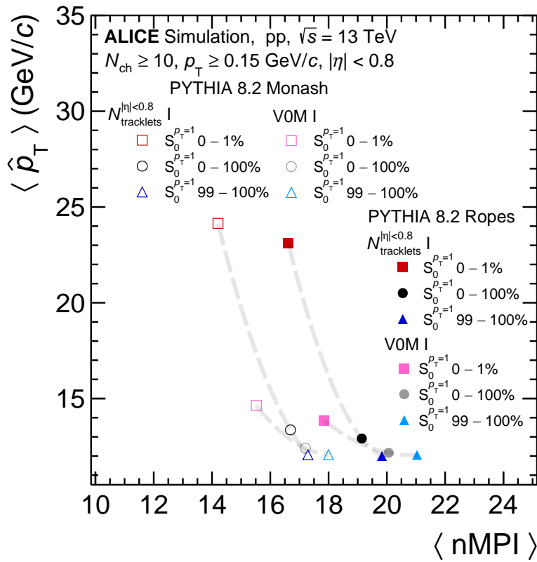
Figure 3: PYTHIA 8.2 correlation study between \langle \hat{p}_T \rangle and \langle n\text{MPI} \rangle as a function of S_0^{p_T=1} , in 0–1% VOM and N_{\text{tracklets}}^{|\eta| < 0.8} multiplicity classes. The default PYTHIA 8.2 Monash variation is compared to PYTHIA 8.2 with color rope hadronization. The total systematic and statistical uncertainties are smaller than the marker sizes. The grey band is an interpolation between the points, to more clearly illustrate the trend of each multiplicity and model variation.
