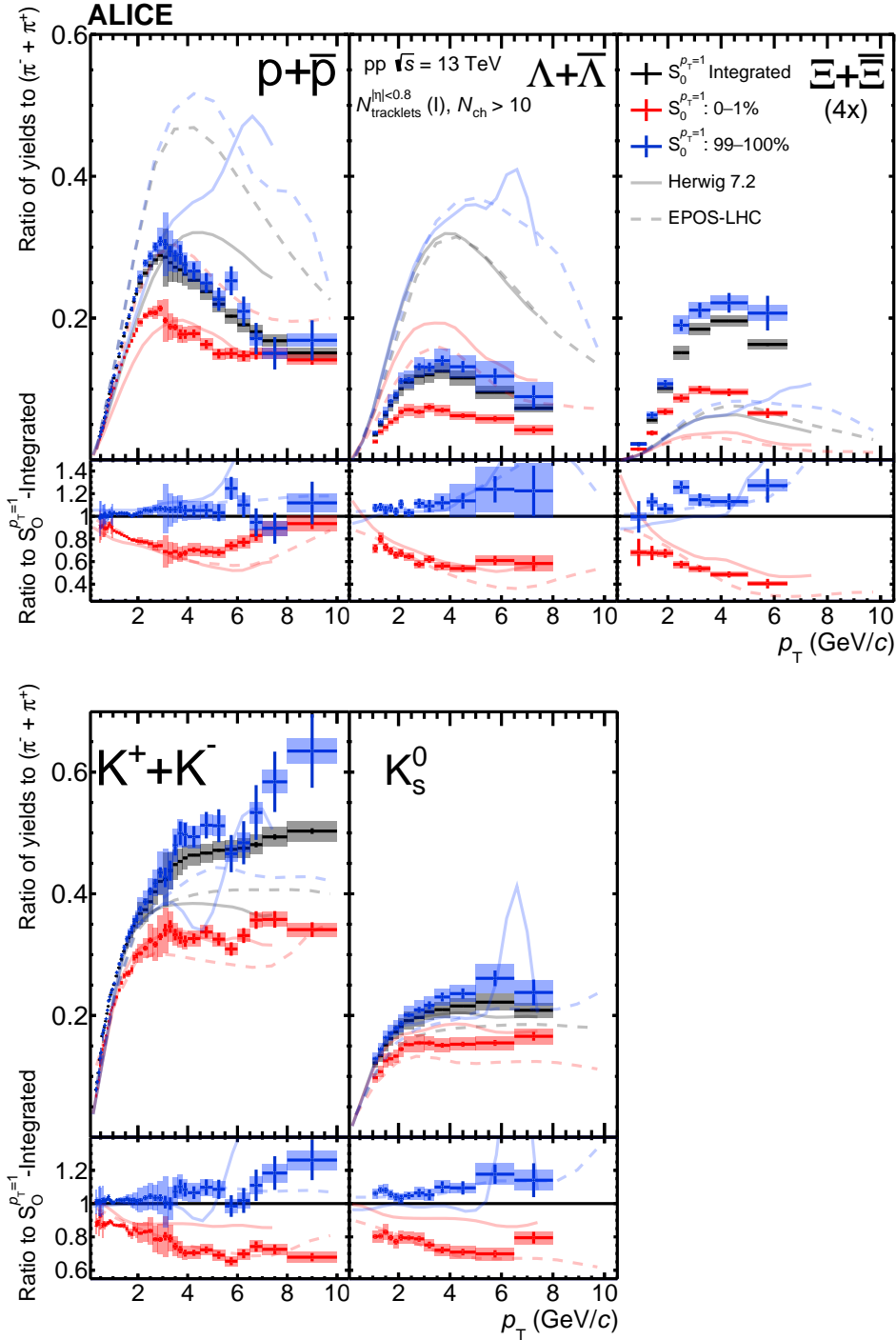
Figure 10: Top panels show hadron-to- \pi ratios for 0–1% S_0^{p_T=1} classes selected for the 0–1% N_{\text{tracklets}}^{|\eta| < 0.8} multiplicity events. Figure 9 and Fig. 10 both contain the same experimental data, but the vertical ranges are modified to accommodate the model predictions. Bottom panels present the hadron-to- \pi double ratios of S_0^{p_T=1} classes relative to S_0^{p_T=1} integrated high-multiplicity events. Statistical and systematic uncertainties are shown by bars and boxes, respectively. Experimental results are compared with predictions from Herwig 7.2 and EPOS-LHC. The large fluctuations present in the Herwig 7.2 predictions are due to statistical limitations.
