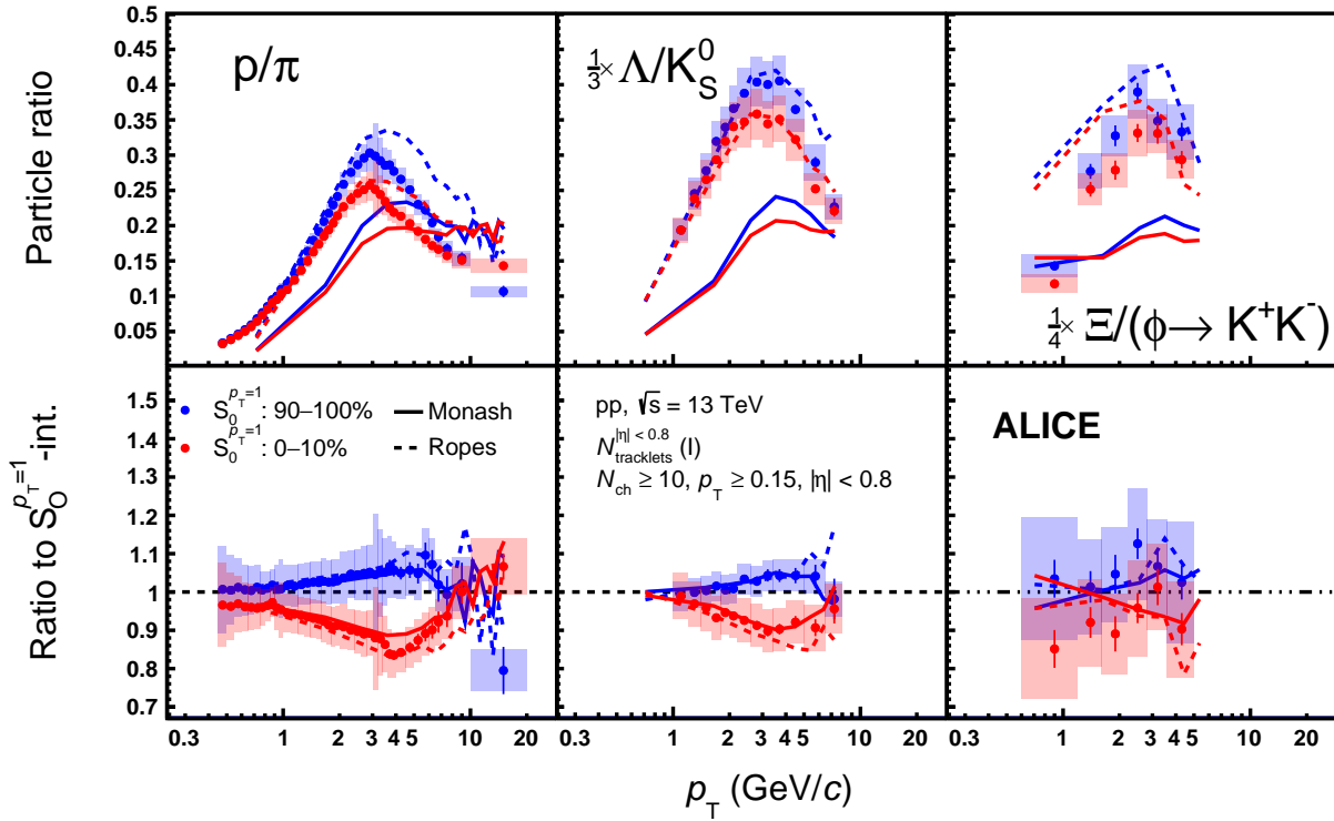
Figure 11: p/\pi , \Lambda/K and \Xi/\phi ratios for different S_0^{p_T=1} classes are obtained for 0 – 1% events measured by N_{\text{tracklets}}^{|\eta| < 0.8} . Lower panels show the ratio to S_0^{p_T=1} -integrated event selection. Statistical and total systematic uncertainties are shown by bars and boxes, respectively. The curves represent different model predictions of the same measurement. Note that for the p/\pi , the same data points are presented in 7, with an extended p_T range now covering 10–20 GeV/c.
